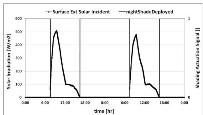
Figure 11 Simulation results showing the solar radiation incident on the shading device, and the shade actuation signal computed in the FMU (1 means that the shade is deployed).
