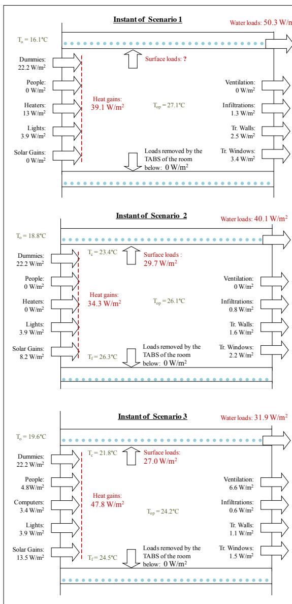
Figure 6 – Instantaneous configuration for the three scenarios.
