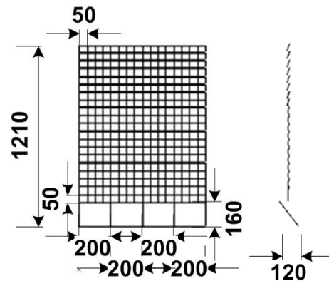
Figure 3 Front and side views of the modelled individual VNLS with simple view and directional light, with an upper tilt angle of 40°
