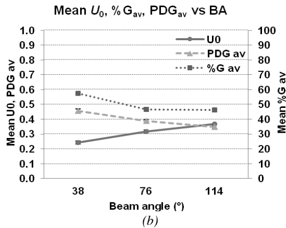
Figure 8 Graphs showing the relationship between the arithmetic mean of the output variables and the most influential input variables, i.e. (a) the space availability and (b) the beam angle. The error bars indicate 95% confidence level.
