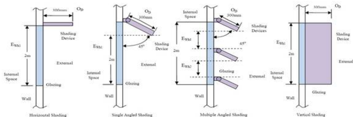
Figure 2- Common Forms of External Solar Shades
