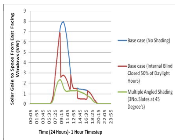
Figure 6- Optimum Shading Device, Internal Blind effect and Basecase Solar Heat Gain for East Facing Window/Shading
