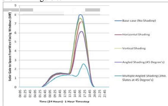
Figure 7- Solar Heat Gain for West Facing Windows/Shading
