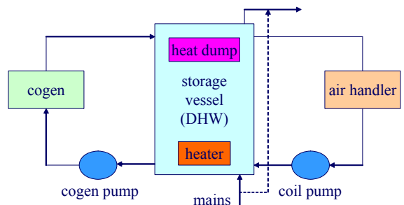
Figure 1 Schematic overview of the SE and SOFC residential cogeneration systems
