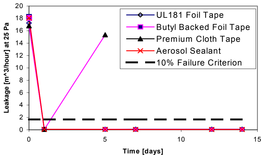
Figure 2b. Changing test sample leakage at 25 Pa from the aging apparatus
