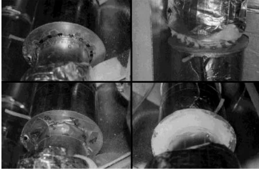
Figure 5. Four samples connections for the aging test. Clockwise from top left: clear UL 181B tape, aerosol sealant, mastic and 181B-FX duct tape.
