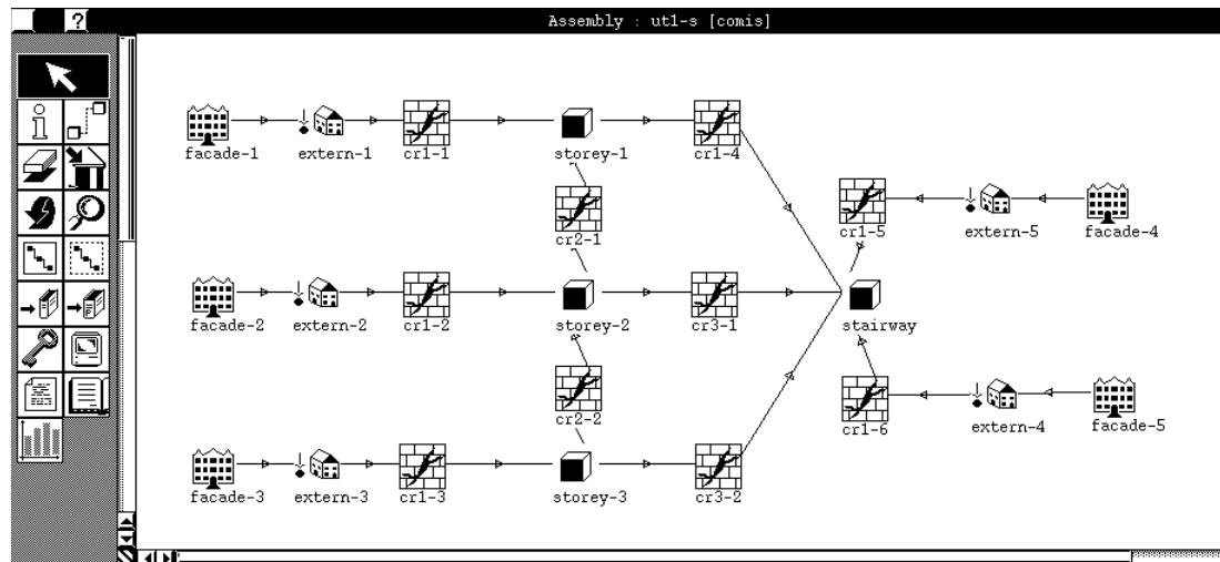
Figure 14: Air-flow network for a three-story building with a common staircase (Keilholz 1997)
