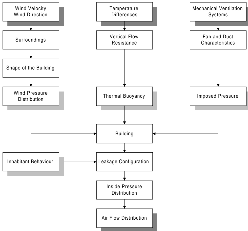
Figure 4: Influences on the Air-Flow Distribution in Buildings (Feustel 1984)
