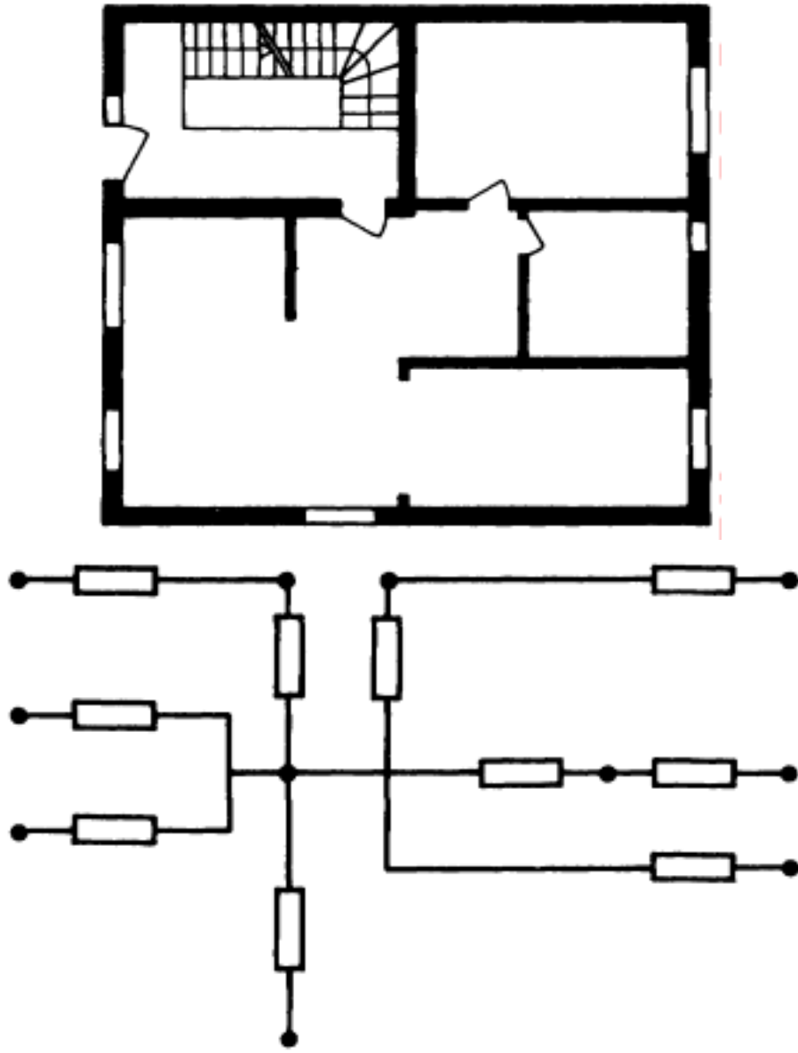
Figure 2: Floor plan of a simple building and its representation in a two-dimensional nodal Network (Feustel 1984)
