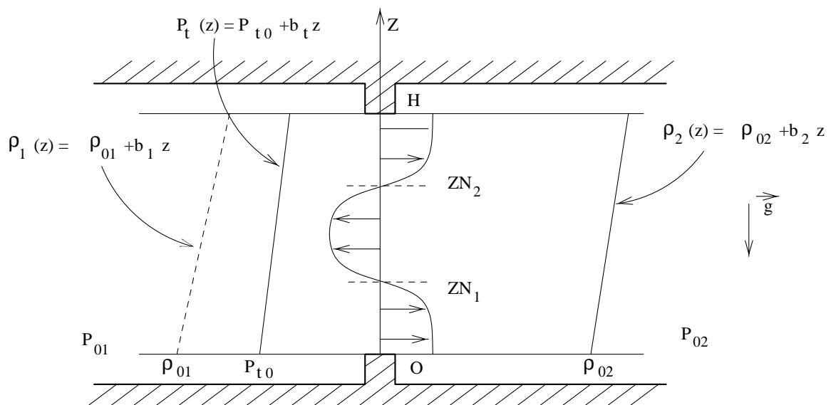
Figure 9: Description of the general problem of gravitational flow through vertical large openings; Index 0 = Reference Height, Index 1 = Zone 1, Index 2 = Zone 2, Index t = effect of turbulence (Allard and Utsumi 1992)
