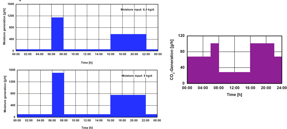
Fig.1: Daily course of moisture generation (left) in the model apartment without (above) and with drying of laundry (below), as well as the course of CO 2 production (right).
