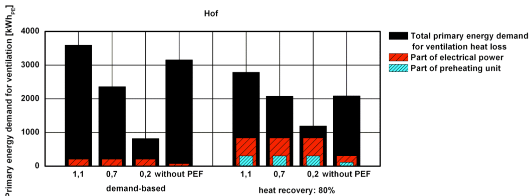
Fig. 3: Energy demand of supply and exhaust ventilation system with heat recovery of 80 % (right) compared to a demand-based exhaust ventilation system (left) by considering primary energy factors.
