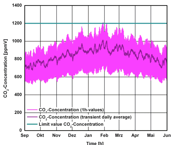
Fig. 4: Course of the CO 2 concentration in a 3-person household using the demand-based exhaust ventilation system as 1-h-values and transient daily average for Hof.
