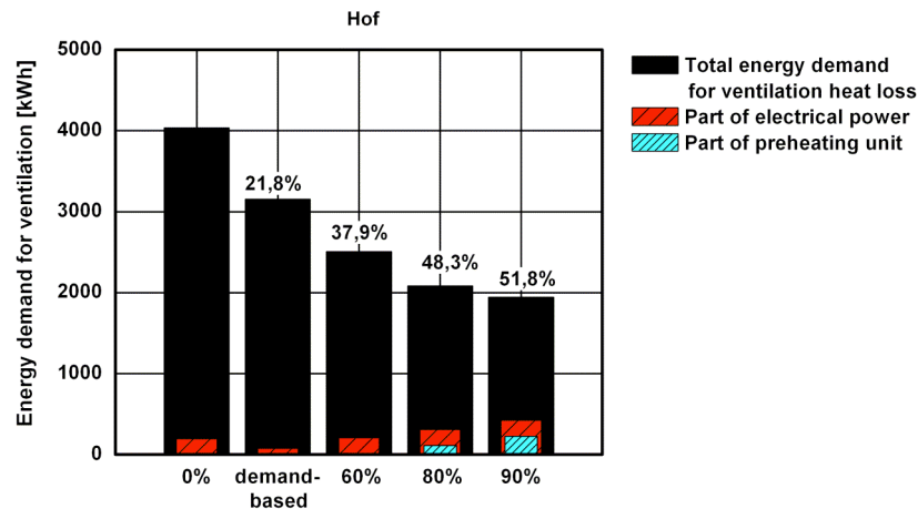
Fig. 2: Total energy demand for ventilation in case of a supply and exhaust ventilation system with a different heat recovery coefficient and in case of a demand-based exhaust ventilation system
