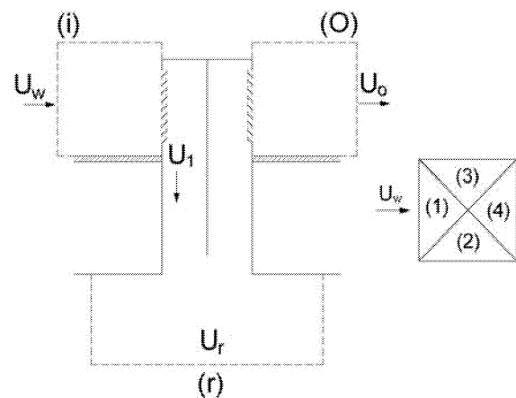
Figure 3: Windcatcher with Control Volume and Plan
