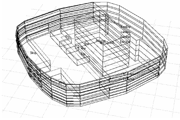
Figure 2: Model of the technical library in ESP-r software
