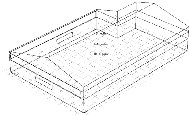
Figure 1: Model of the hall in ESP-r
