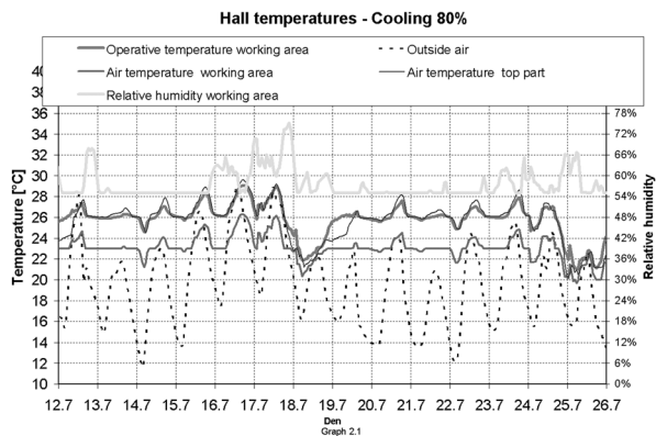
Figure 3: Temperatures in the kiln hall variant 2 for selected period
