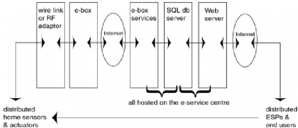
Figure 2: Architecture of the SmartHomes system
