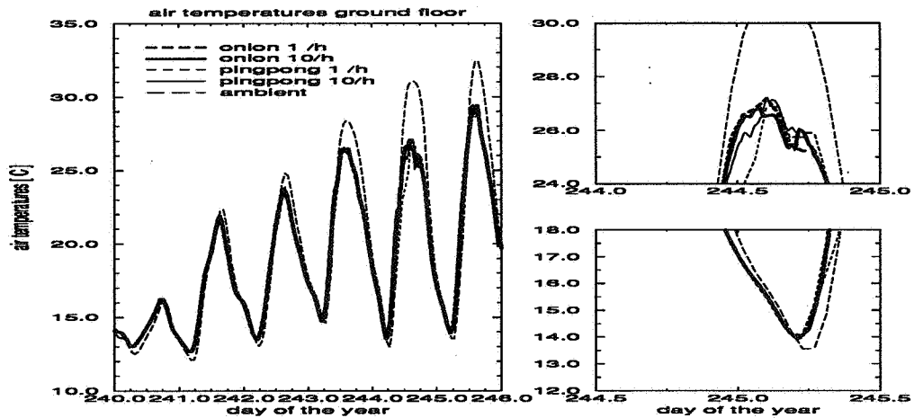
Figure 5 Simulation results for ground floor air temperatures
