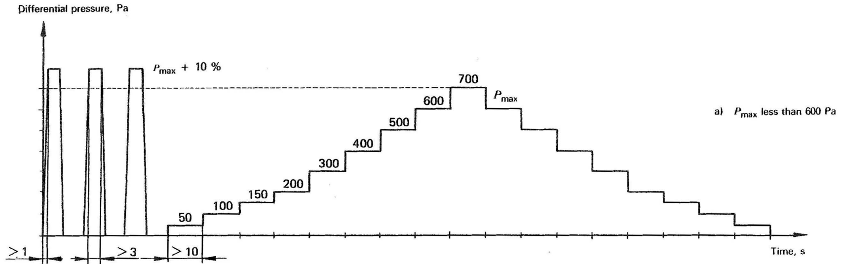
Figure — Sequence of differential pressure application
