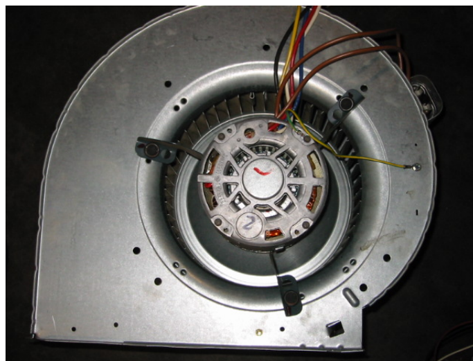
Figure 2. Fan housing inlet with direct drive PSC motor
