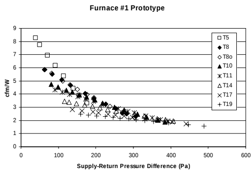
Figure 15. Furnace #1 test results. T numbers are torque settings (5 low to 19 high).
