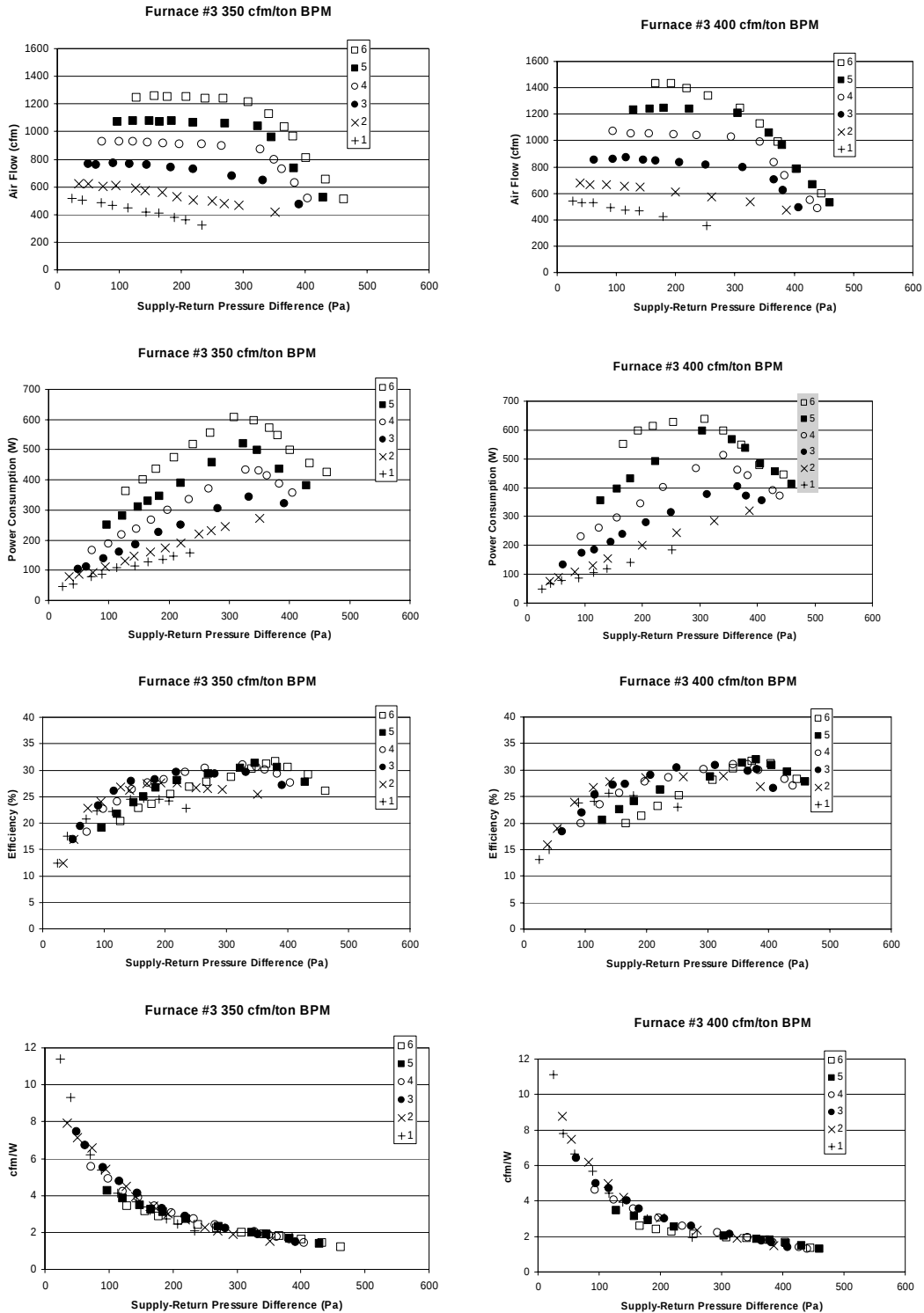
Figure 17. Furnace #3 test results at two different cfm/ton ratings. T numbers are torque settings (5 high to 1 low).
