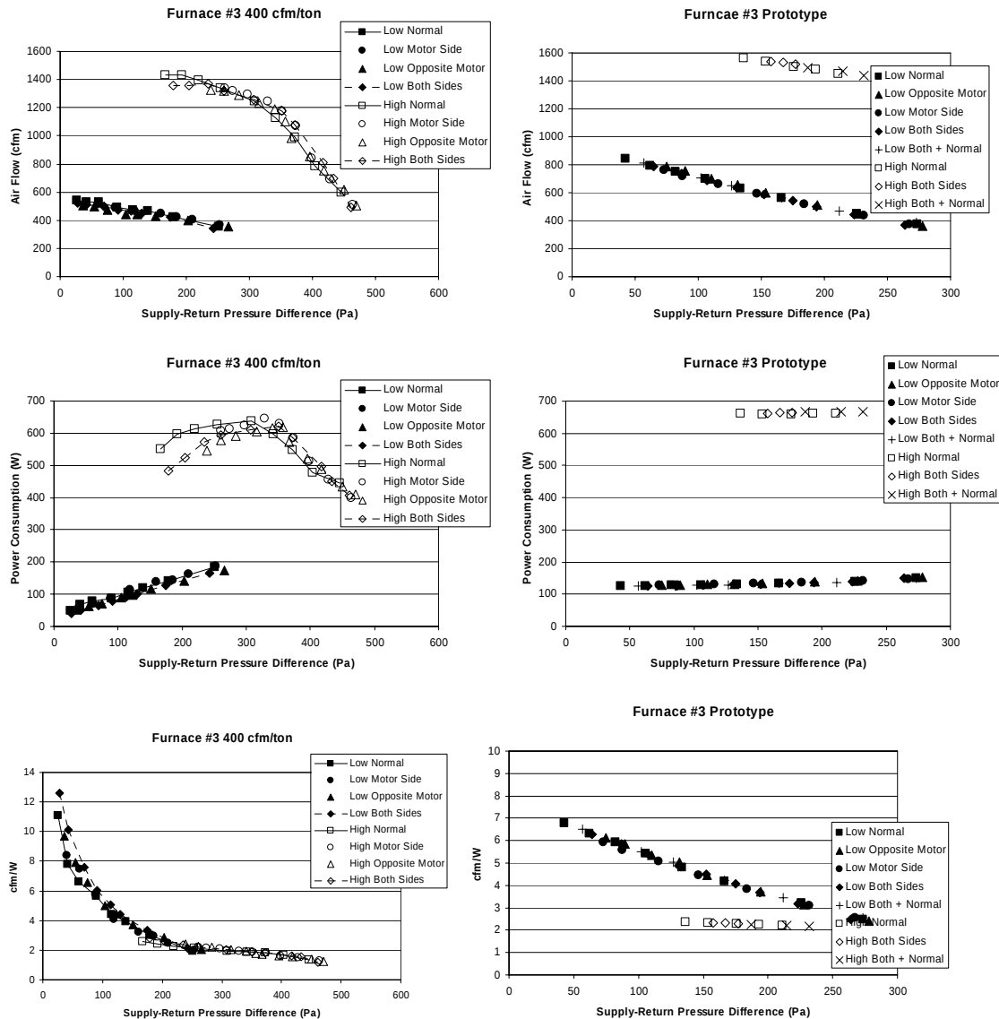
Figure 20. Effect of air inlet location for Furnace #3
