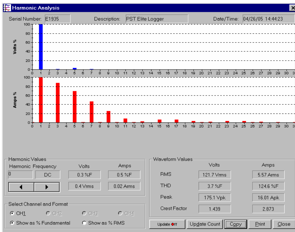
Figure 28. Wave form and harmonic analysis for Furnace #2 prototype BPM motor, torque setting 11.
