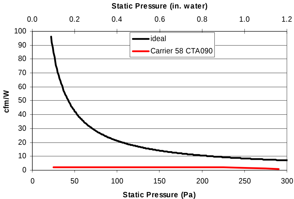
Figure 4. Maximum theoretical cfm/W for different static pressures compared to a typical residential unit
