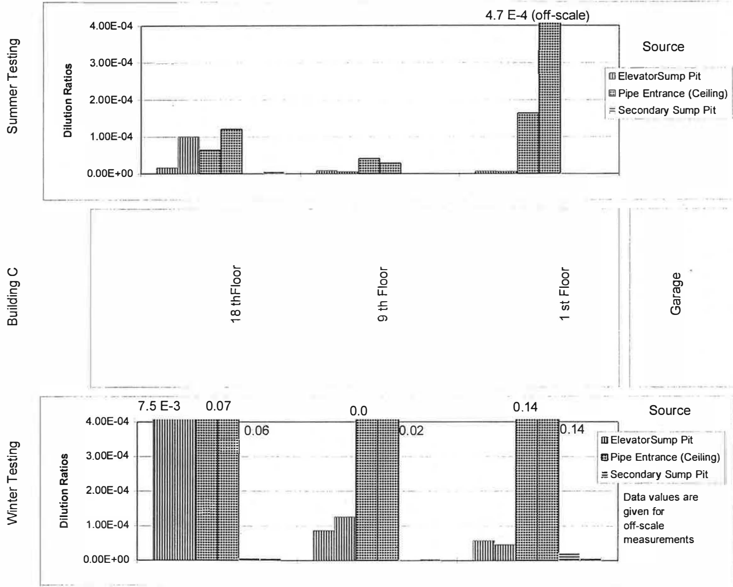
Figure 5.2.6 PFT Dilution Ratios in Living Space
