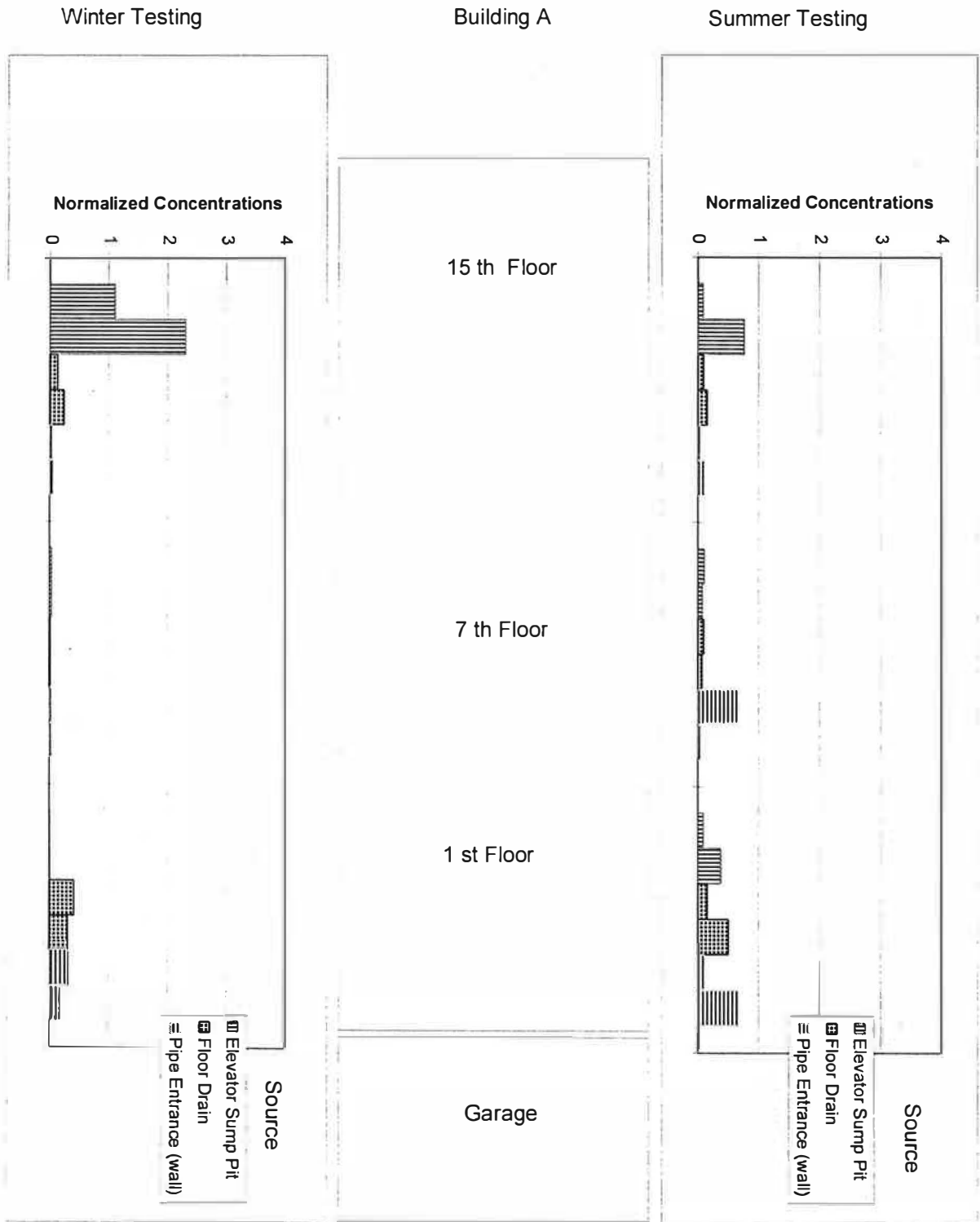
Figure 5.2.1 Normalized PFT Concentrations in Living Space
