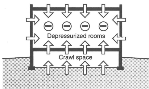
Figure 1-4: Some mechanical ventilation systems are not properly balanced resulting in depressurization of the interior spaces in a building. This can induce radon to enter spaces and must be addressed in a mitigation effort.
