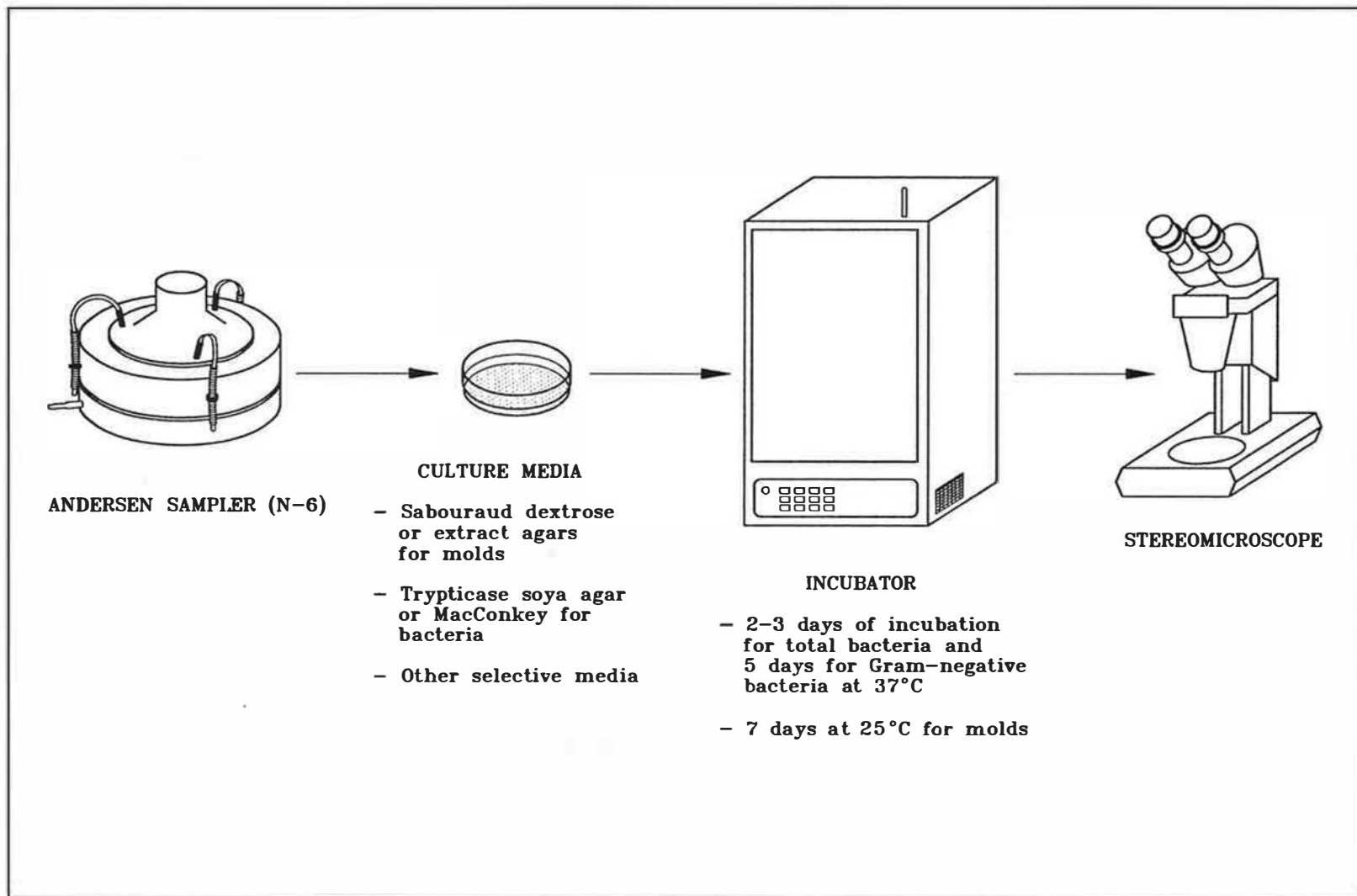
Figure 4.5: Sampling and analytical method used at the IRSST
