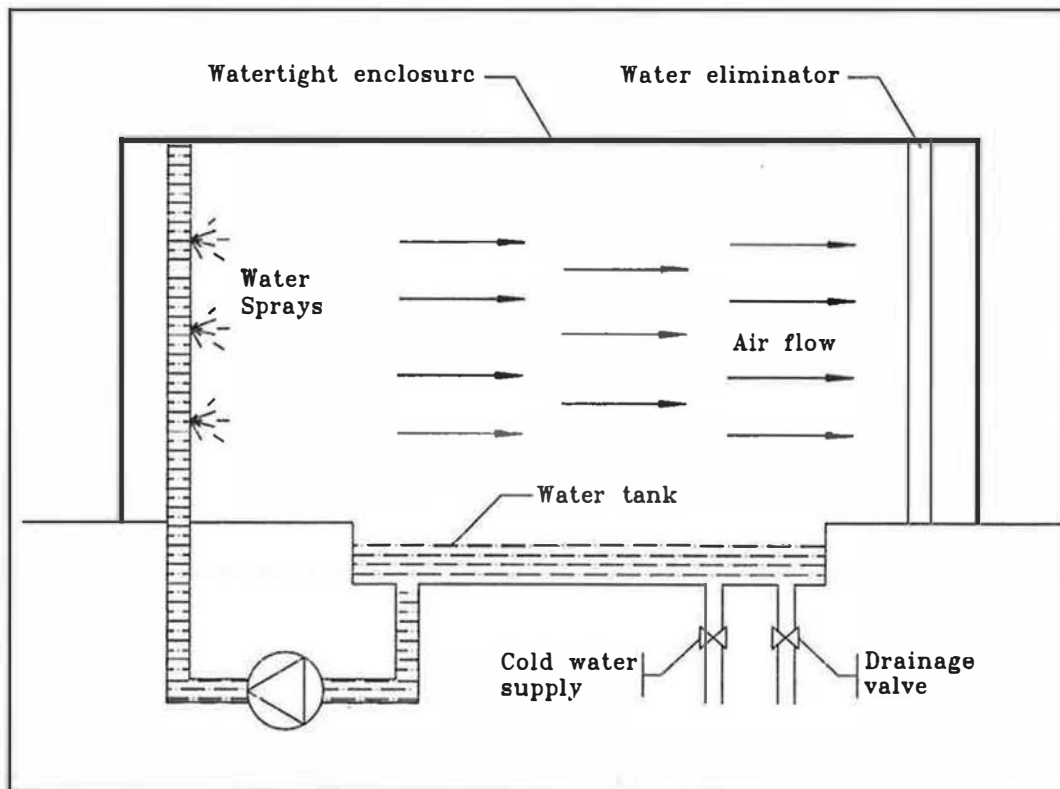
Figure 3.12: Diagram of a spray humidifier
