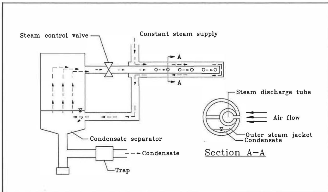
Figure 3.8: Diagram of a dry steam humidifier
