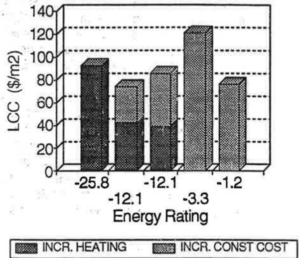
Fig. 2 Example Result: Life Cycle Cost of Window Options
