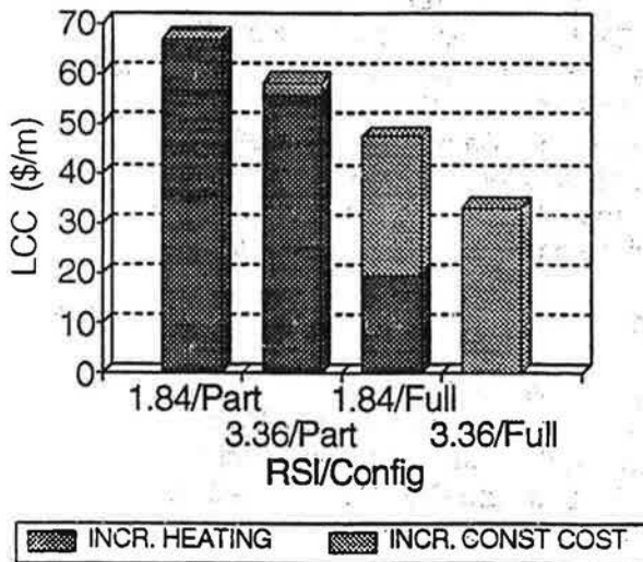
Fig. 3 Example Result: Life Cycle Cost of Below Grade Wall Insulation Options.
