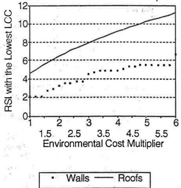
Fig. 4 Effect of the Environmental Cost Multiplier on the Selection of Envelope Thermal Characteristics
