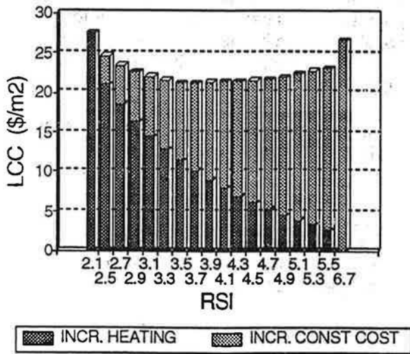
Fig. 1 Example Result: Life Cycle Cost of Wall Options
