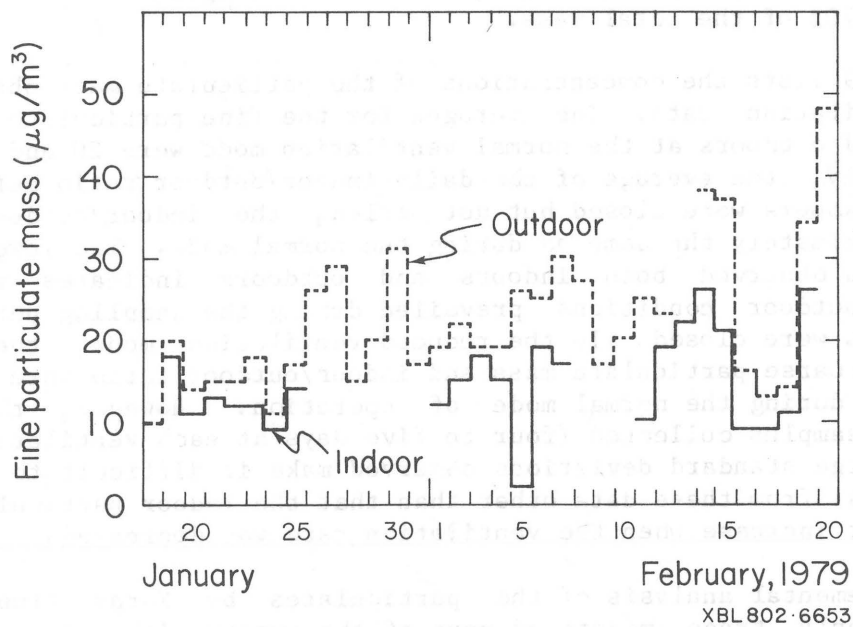
Figure 12. Comparison of particulate mass in Room 12 and outdoors during January and February, 1979.
