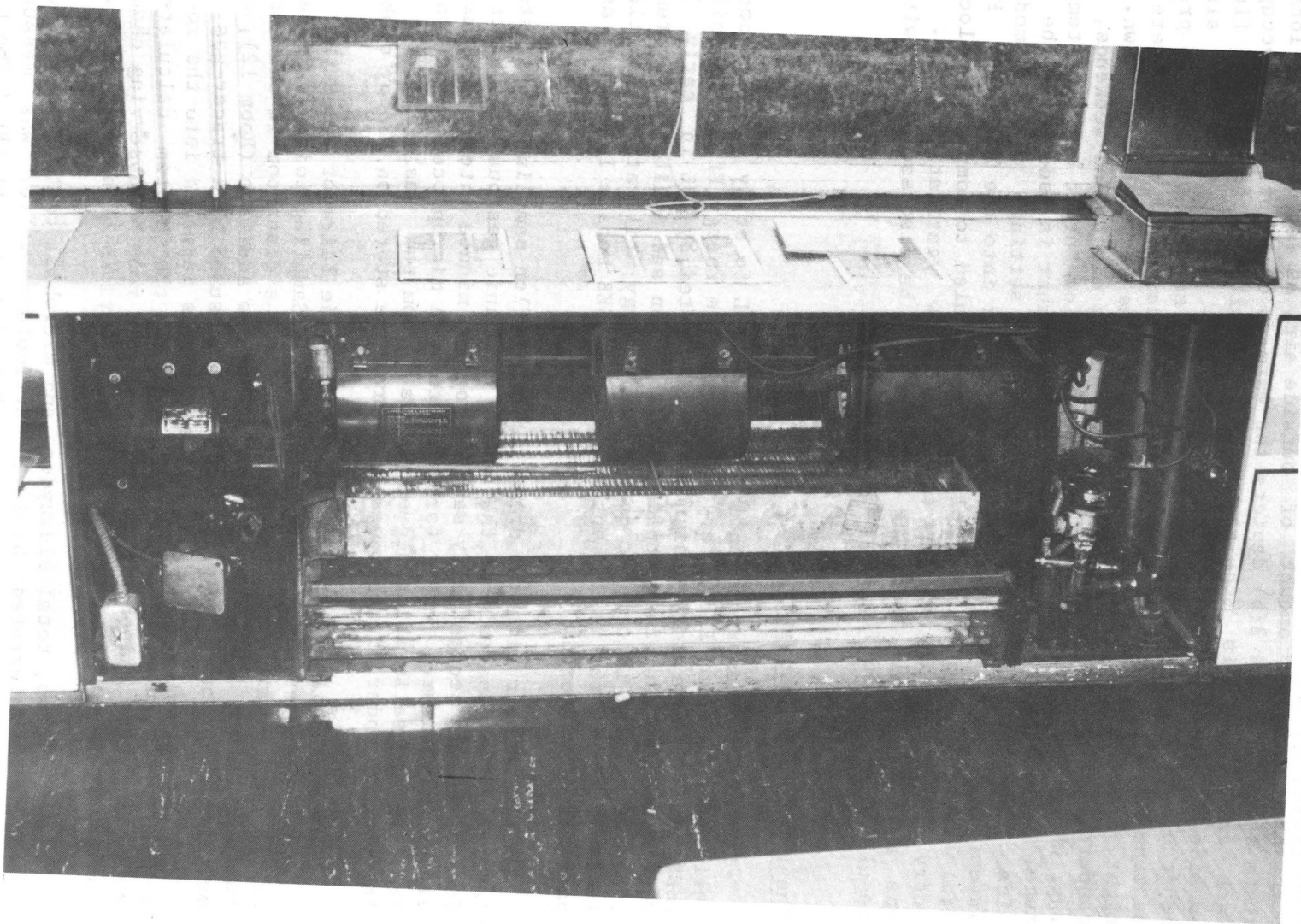
Exhibit 1b. View of the unit ventilator without the front panel.
