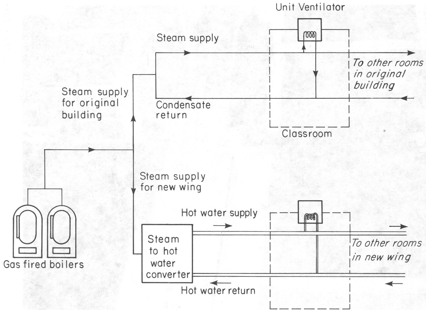
Figure 2. Schematic of the heating system at Fairmoor Elementary School.
