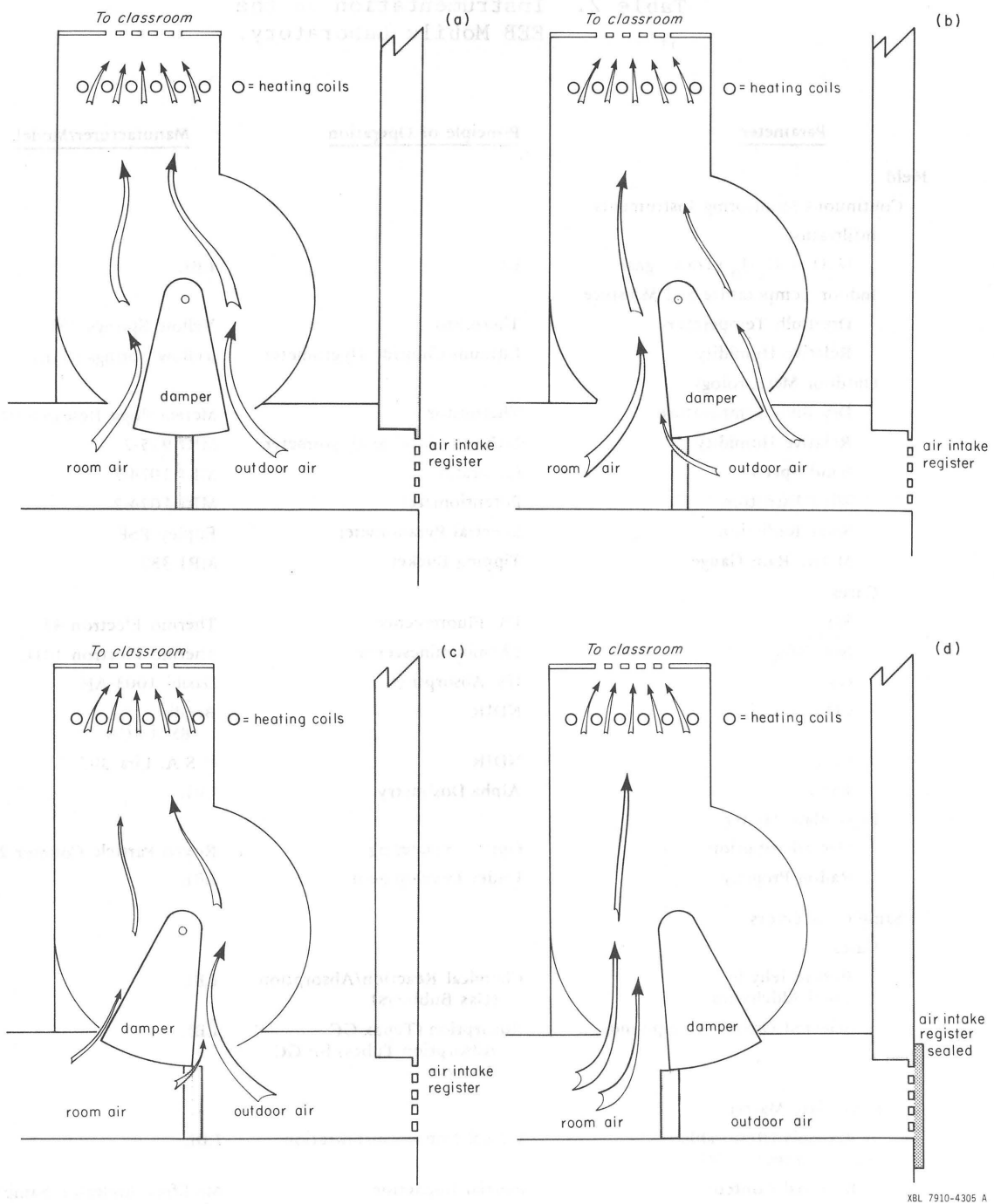
Figure 3. Damper position and air flow in various modes of operation of the unit ventilators:
