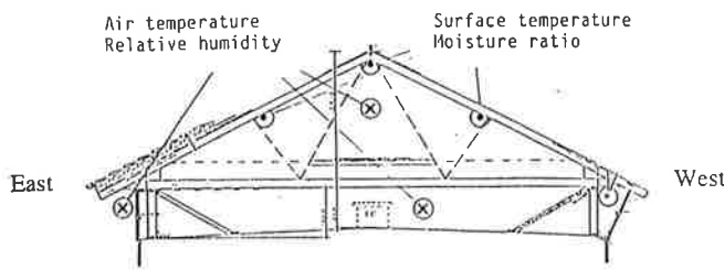
Figure 5 Schematic arrangement of sensor positions.
