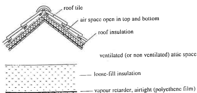
Figure 1 If the outside of the inner roof layer is insulated, the inner roof layer itself and the roof space will become somewhat warmer and dryer. If, in addition, inner roof ventilation is reduced or stopped entirely, there will no longer be the adverse effects that can arise from ventilation, particularly during cold, clear nights. However, stopping ventilation entirely involves a risk of damage if moisture finds its way into the roof space.
