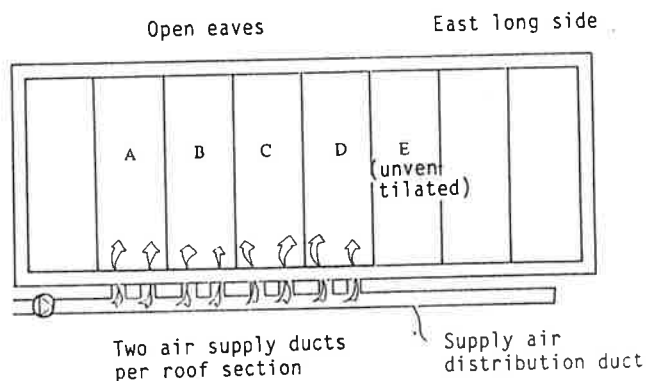
Figure 4 Plan of the roof spaces.
