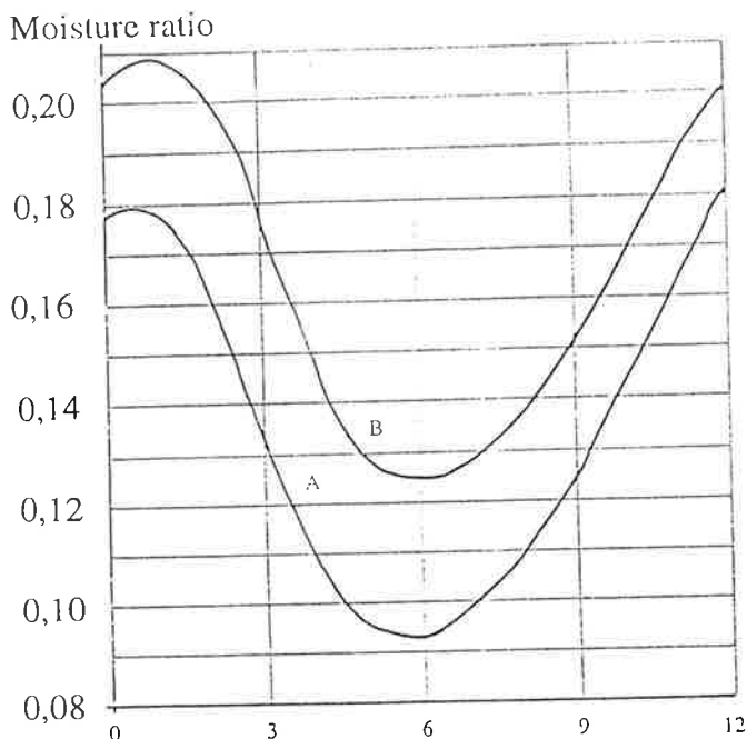
Figure 3 Calculated moisture ratio in the inner roof layer over a period of one year. Curve A indicates normal conditions, and curve B indicates a roof without solar input.
