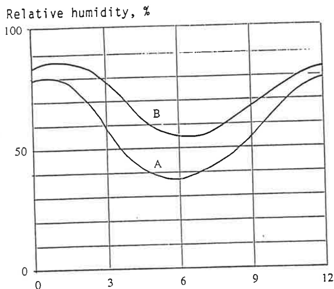
Figure 2 Calculated mean relative humidity in a roof space over a period of one year. Curve A indicates normal conditions, and curve B indicates a roof without its solar input. Measured values during a year should fall between the two curves.
