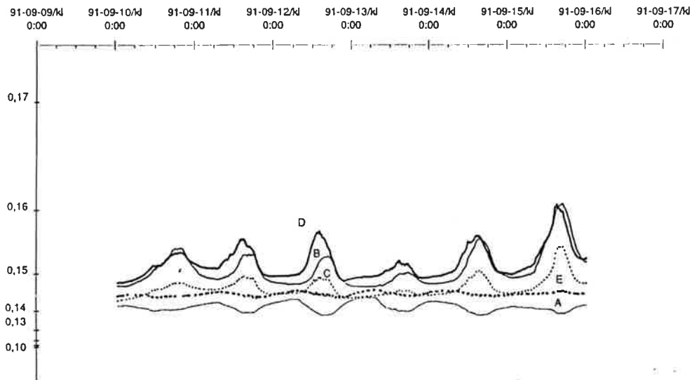
Figure 8 Moisture ratios in the inner roof structure of the five roof spaces during the period September 9-16, 1991. The moisture ratio in roof space A has been measured about 1 cm from the plastic film (Monarfol) on the upper side of the joist. Values are expressed as mean values of the three measurement points in the roof space.
