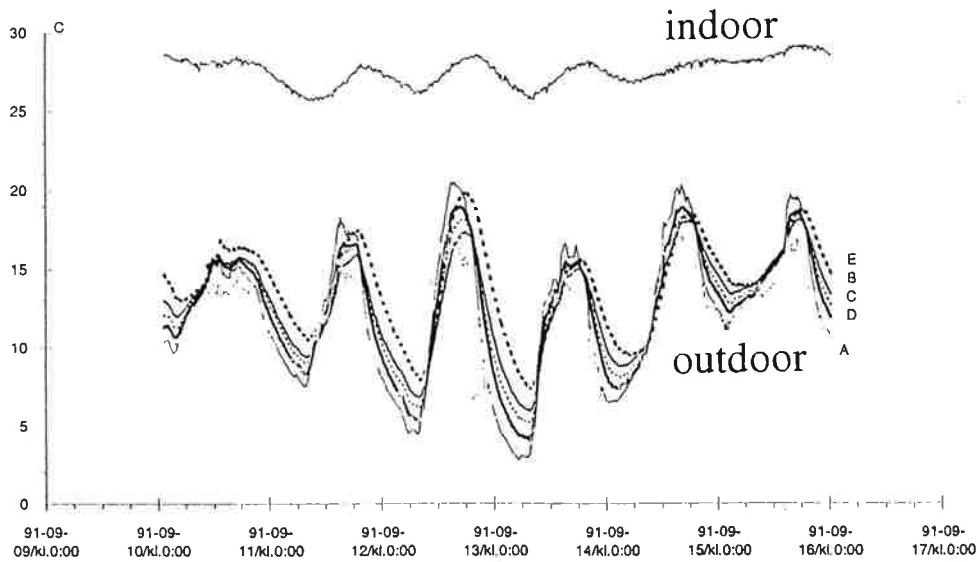
Figure 7 Air temperatures in the five roof spaces, outdoors and indoors, September 9-16, 1991.
