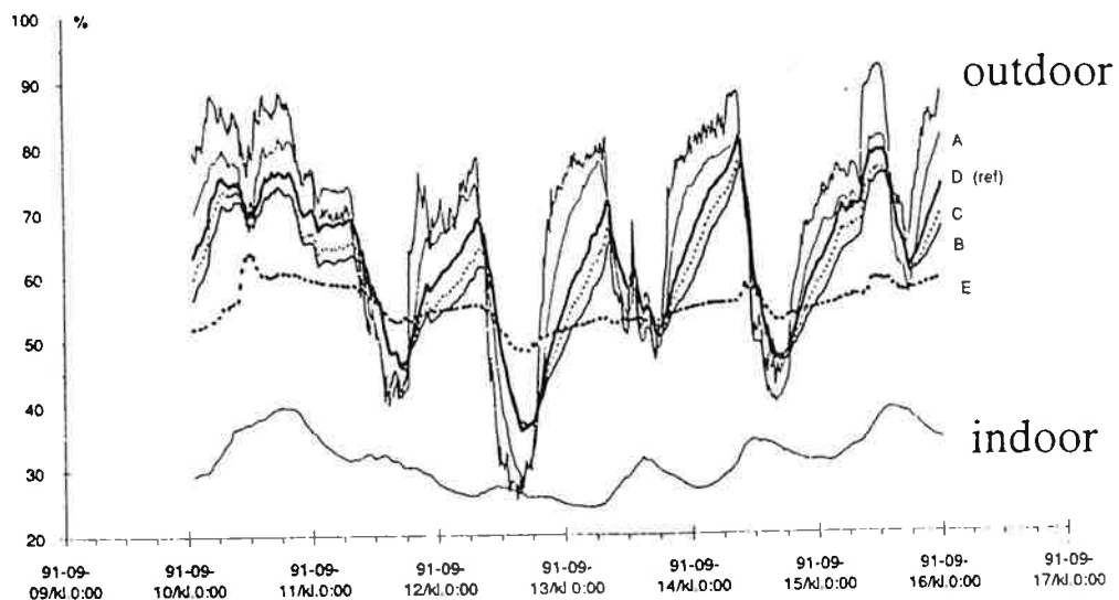
Figure 6 Relative humidity in the five roof spaces, outdoors and indoors, September 9-16, 1991.
