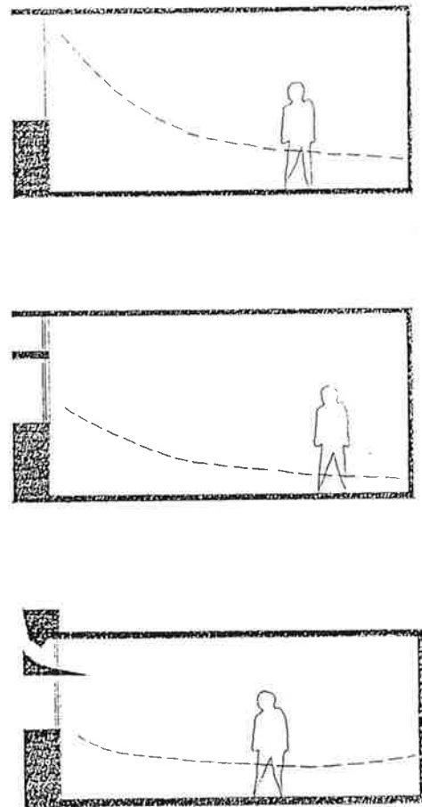
Figure 6 Light distribution analysis for first candidate demonstration building, comparing (top to bottom) a simple window, a standard light shelf, and the proposed "passive optical light shelf" for an east orientation facade. Room section is shown for each option with horizontal daylight illumination measured at workplane height plotted through the section. Note the third option has the most uniform distribution and thus implies an environment with less potential for window glare. Measurements reflect clear day solar conditions at 9 a.m. on September 21 at latitude 34°N.
