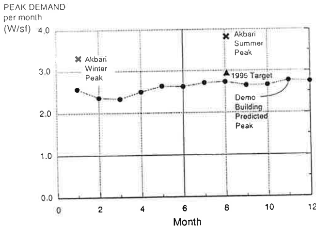
Figure 5 Computer-simulated performance of the first candidate demonstration building, compared to our 1995 target value for Los Angeles (Sullivan et al. 1992) and compared to data from a simulation study of existing Los Angeles office building performance (Akbari et al. 1989).
