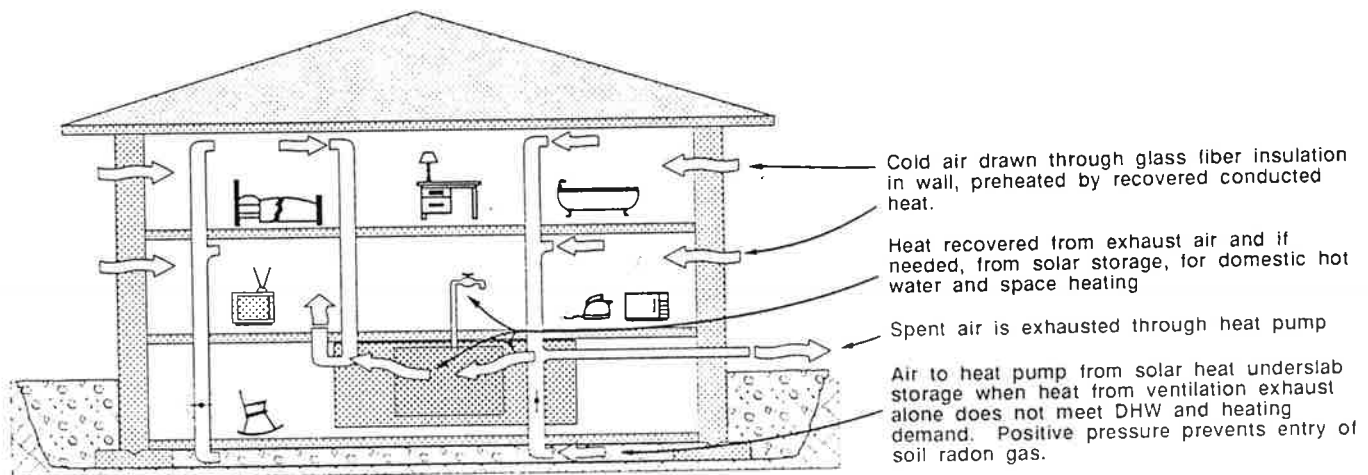
Figure 6 Operation of a house during nighttime or cloudy conditions.
