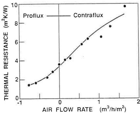
Figure 1 Effective thermal resistance plotted against dynamic airflow rate.
