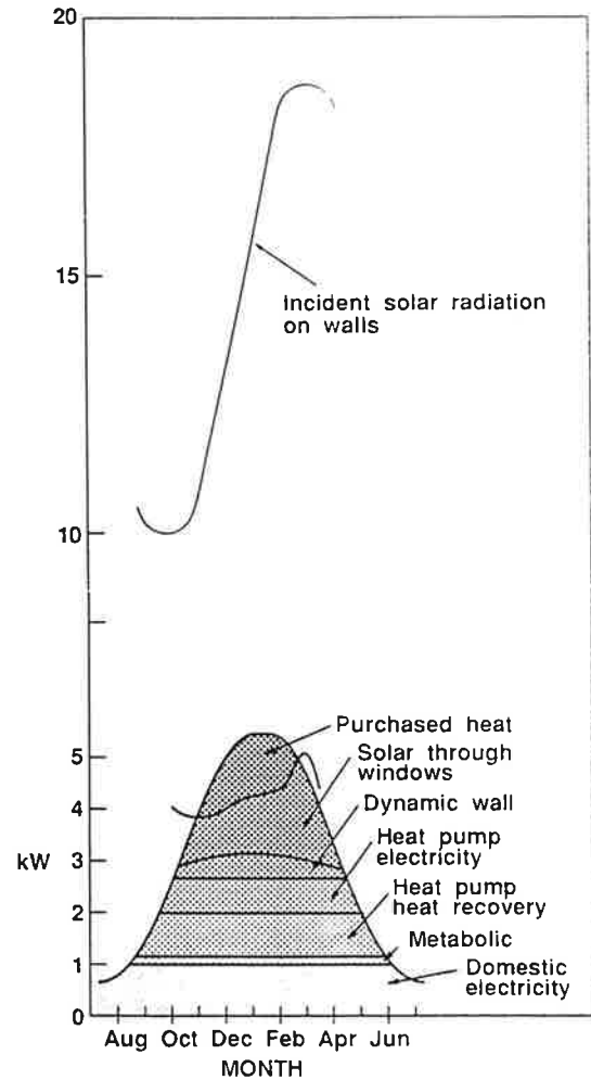
Figure 4 Energy demand (heating, ventilating, domestic hot water) and energy supply plotted against the months of the year.
