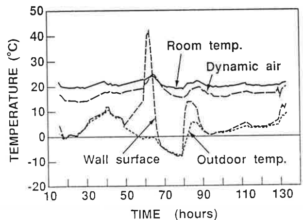
Figure 2 Indoor air temperature, dynamic air temperature, wall surface temperature and outdoor air temperature plotted against time in hours. Note sharp wall surface temperature peak during bright sunny conditions.
