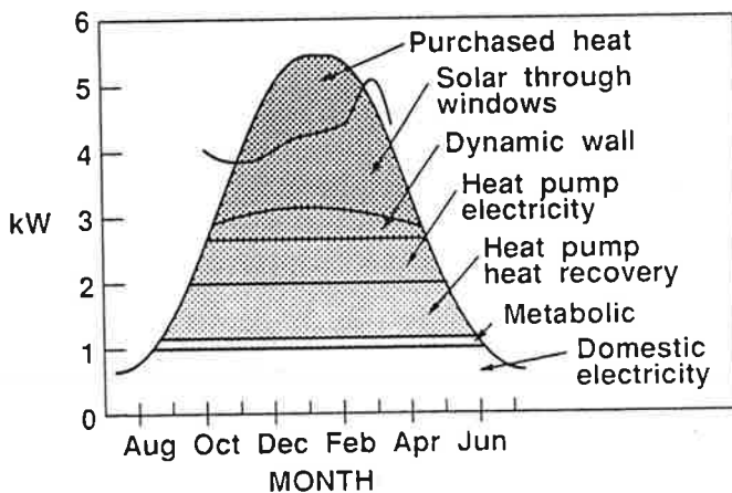
Figure 3 Energy demand (heating, ventilating, domestic hot water) and energy supply plotted against the months of the year.
