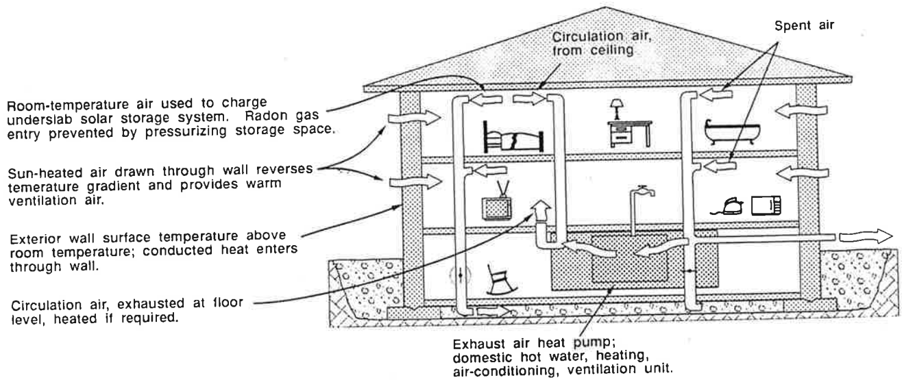
Figure 5 Operation of a house during sunny conditions.
