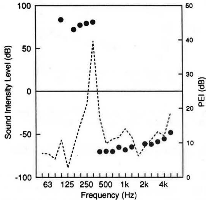
Figure 7: Intensity measurements in the small reverberation room on the horizontal surface of the duct. The loudspeaker was the source.
