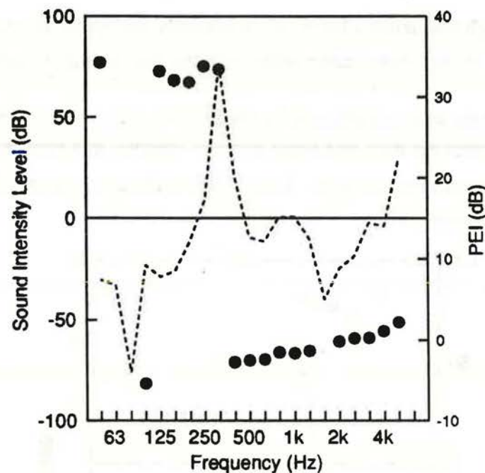
Figure 8: Intensity measurements in the small reverberation room on the vertical surface of the duct. The loudspeaker was the source.
