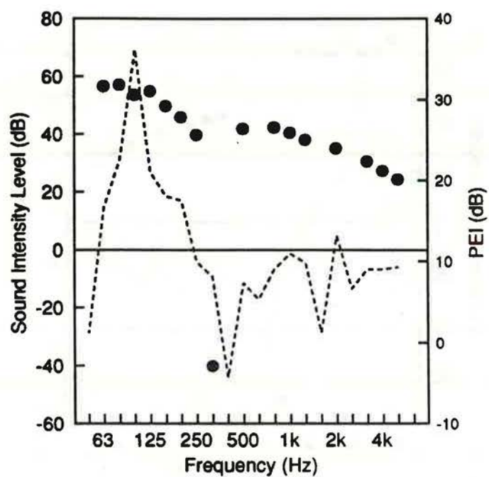
Figure 13: Intensity measurements in the large reverberation room over the horizontal duct surface. The noise source is the fan running unobstructed.
