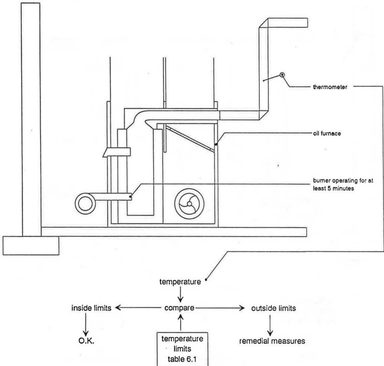
FIGURE 6.1 Oil Chimney Performance Test - Temperature
