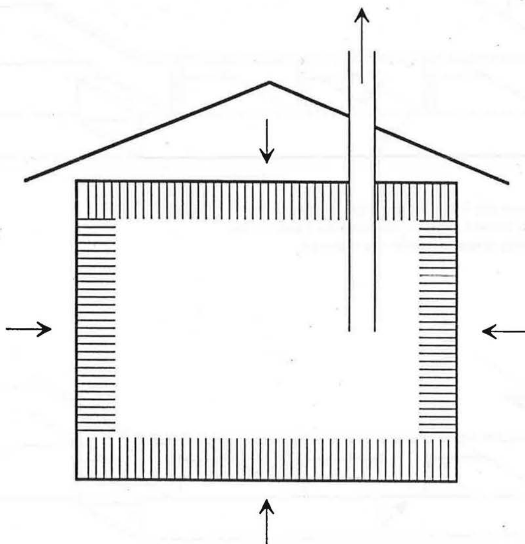
Air Leakage Resulting From Flue and Mechanical Effects
