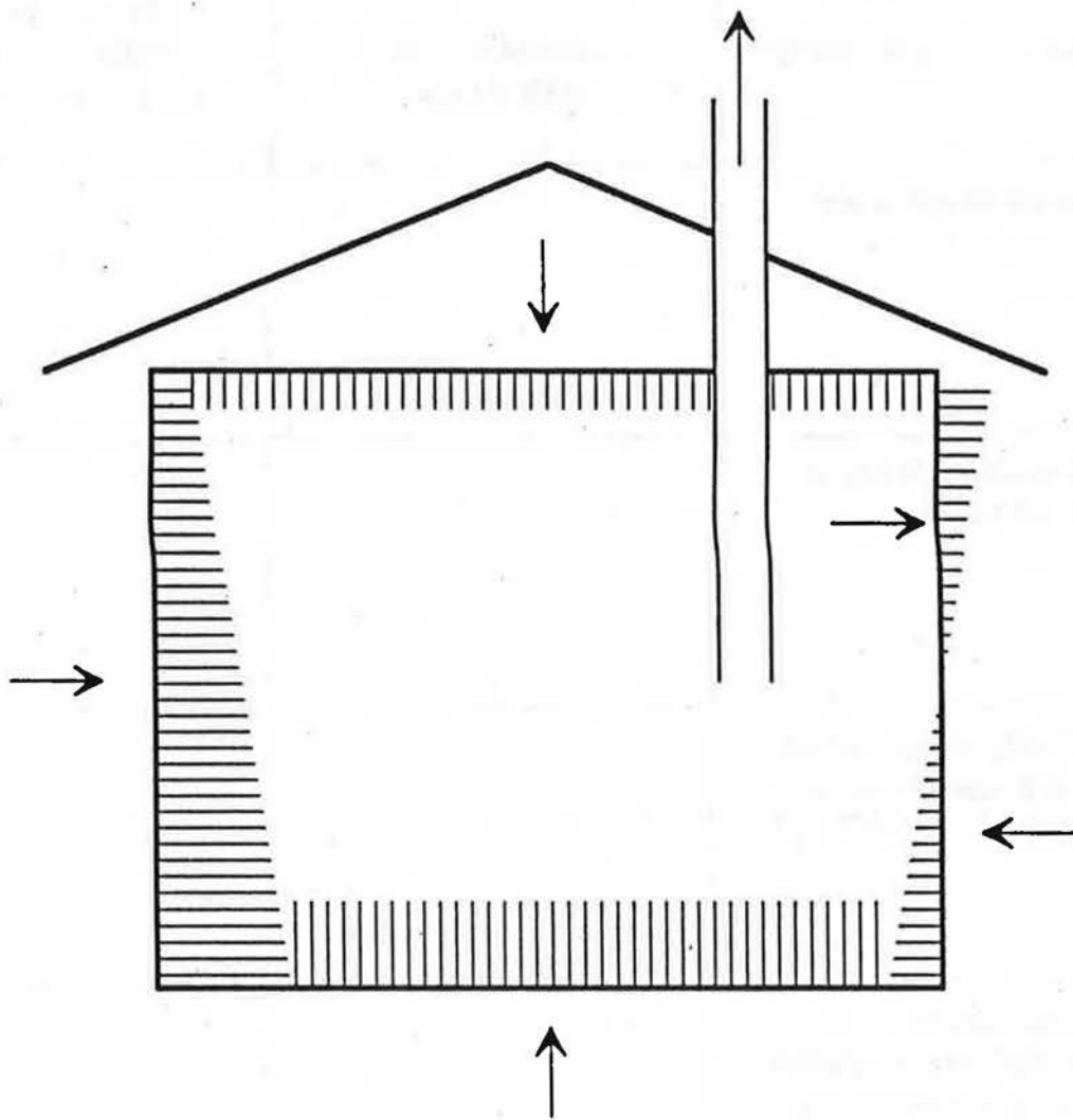
Air Leakage Resulting From the Combined Effect of Stack, Wind and Mechanical Ventilation
