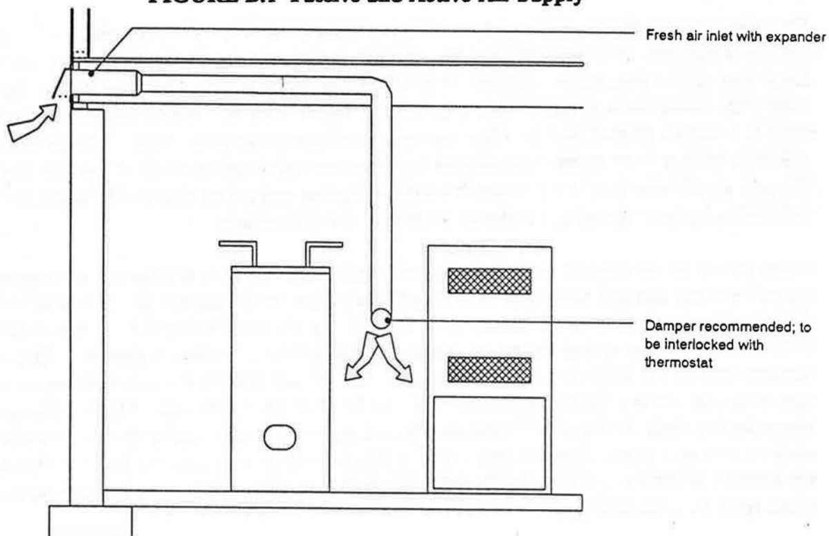
Passive Make-Up Air Duct
