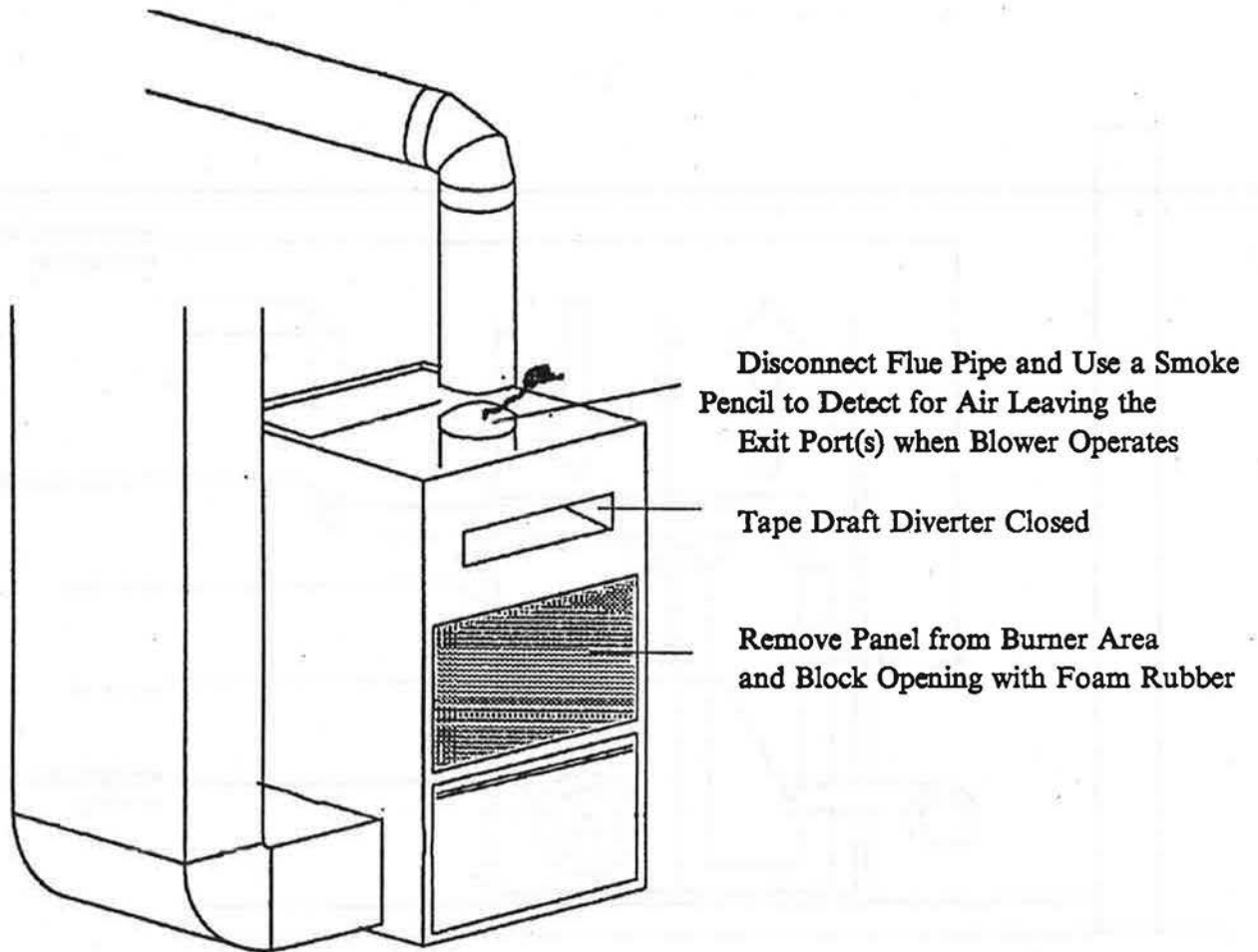
Gas Furnace
