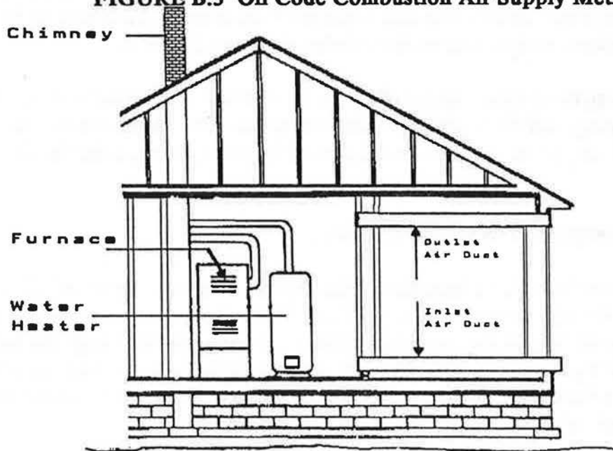
FIGURE B.3 Oil Code Combustion Air Supply Method
