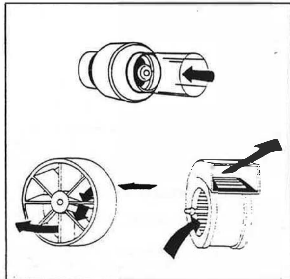
Fan Types : In-line fan (top), axial flow or propeller fan (bottom left), centrifugal or squirrel cage fan (bottom right)
