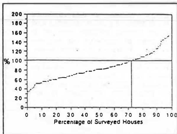
Seasonal Average Air Leakage Rate as % of 1990 Ventilation Requirement [37]
