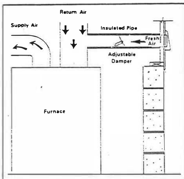
Example of a Fresh Air Supply to Return Air Plenum System [57]
