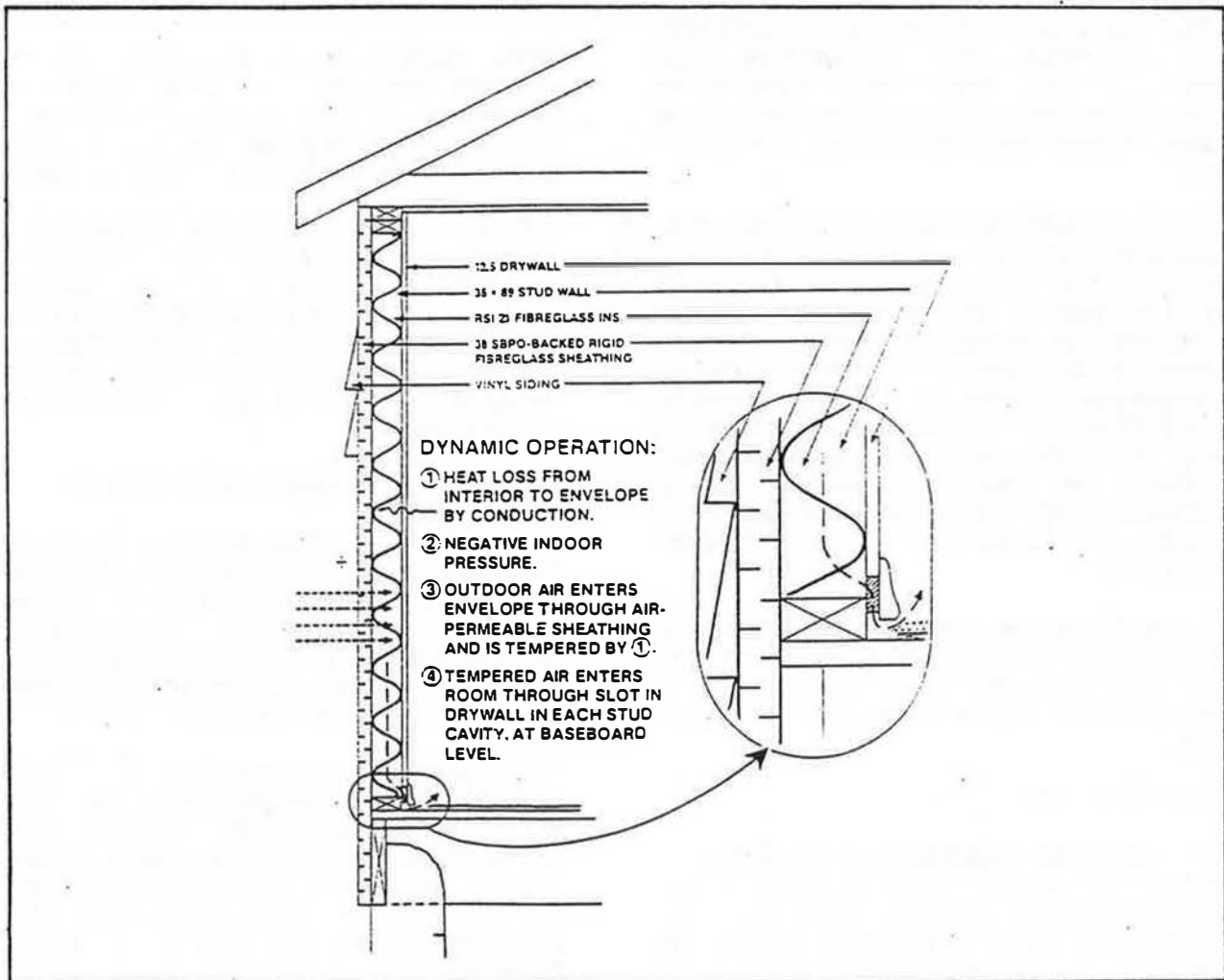
Dynamic Wall Operation [51]
