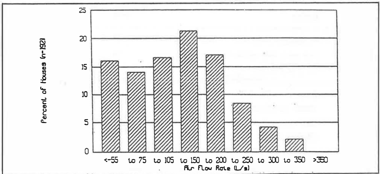
Air Flow Rates Required to Create 5 Pa Depressurization [35]
