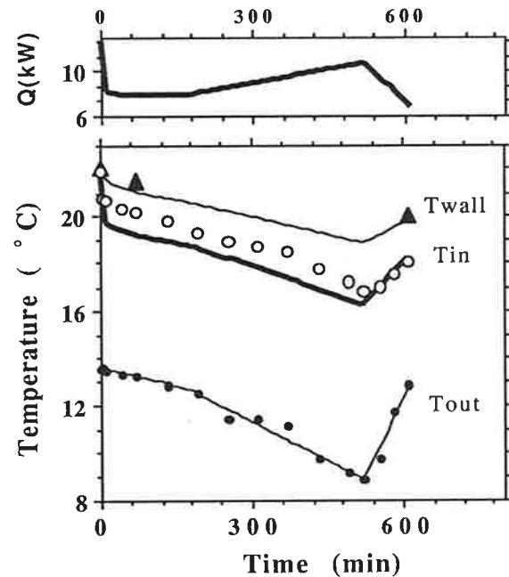
Figure 2. Night ventilation of a 540m 3 staircase from 10 p.m. to 8 a.m. The measured and calculated exhausted inside air temperature, T_{in} , the outside temperature, T_{out} , the wall temperature, T_{wall} , and the calculated heat loss rate, Q , as a function of ventilation time. A_b=1\text{m}^2 , A_t=1.8\text{m}^2 , H=9.6\text{m} . The calculated energy loss over 10 h is 90kWh.
