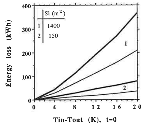
Figure 3. Simulation of energy loss by night time ventilation. Calculated is the total energy loss integrated over 10 hrs, for two values of S_i and b and as a function of initial inside-outside temperature difference, T_w(t=0) - T_{out} ; T_{out} = constant. b=1000 (thick curve), 250 (thin curve) \text{J}/(\text{m}^2\text{Ks}^{0.5}) . A_{in}=2\text{m}^2 [20 ft 2 ]. A_{out}=2\text{m}^2 [20 ft 2 ]. H=10\text{m} [33 ft].
