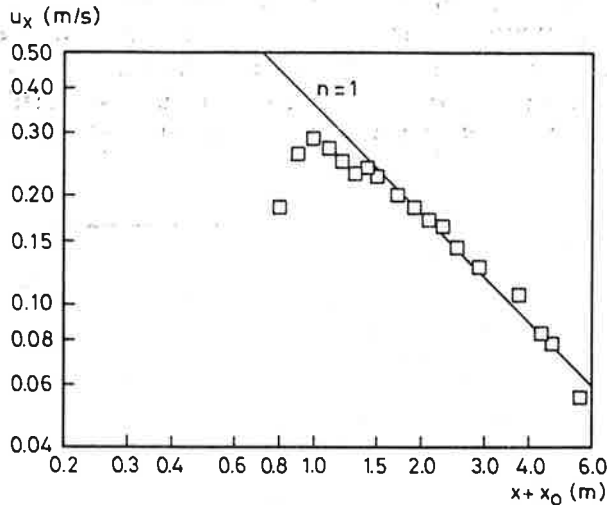
Figure 9. Velocity decay in the flow from diffuser D_1 versus (x + x_0) . q_o = 0.028 m^3/s , Ar = 45.8 and x_o = 0.5 m.
