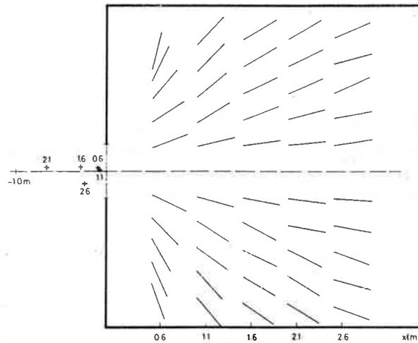
Figure 8. Flow directions at the floor. Diffuser type D_1 . q_0 = 0.028 \text{ m}^3/\text{s} and Ar = 47 . Reference [10].
