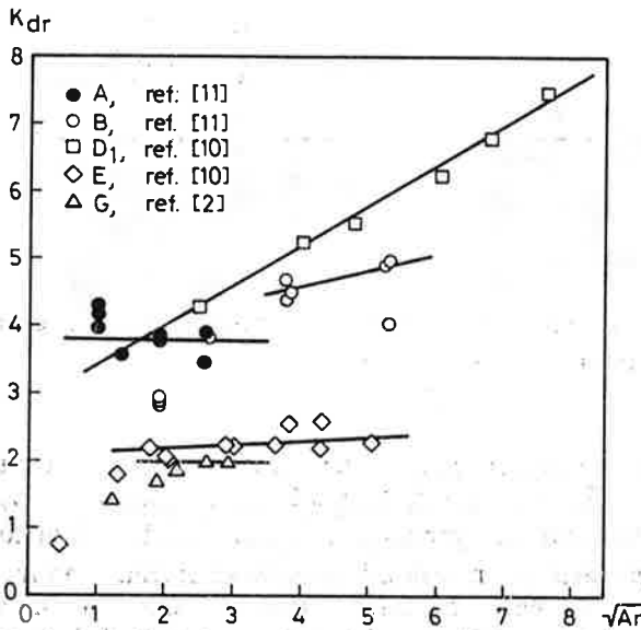
Figure 11. K_{dr} versus Archimedes' number for five different wall-mounted air terminal devices. x_0 = 0.0 .
