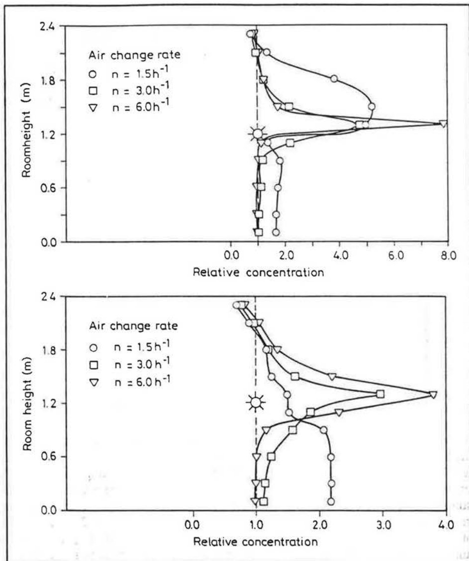
Figure 2. Relative concentration profiles in the middle of the test room for three different air change rates measured with A) a passive tracer gas method and B) a conventional tracer gas method.
