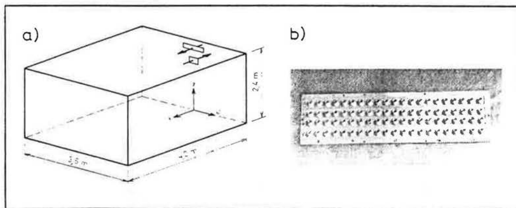
Figur 1. a) Sketch of the geometry of the full-scale test room. b) Close-up of the HESCO inlet device.
