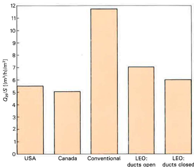
Figure 5 Envelope leakage of office buildings
