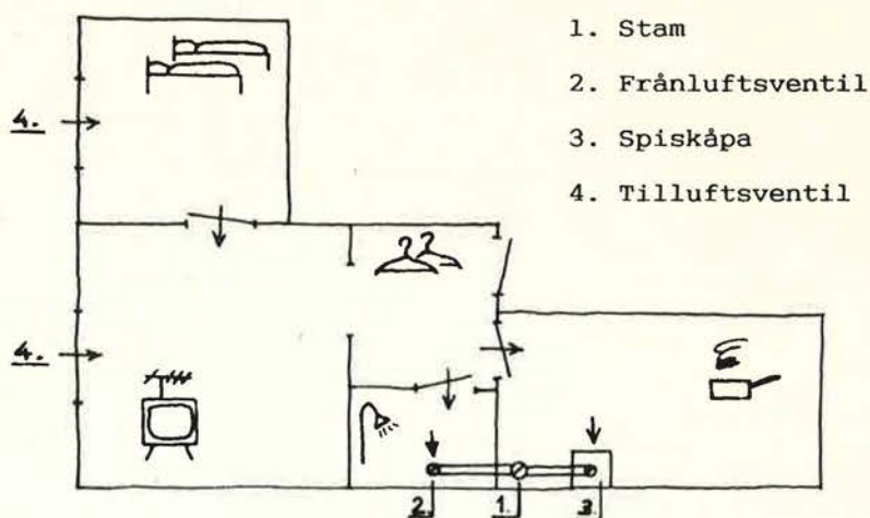
Fig 4. Modelllägenhet, plan
