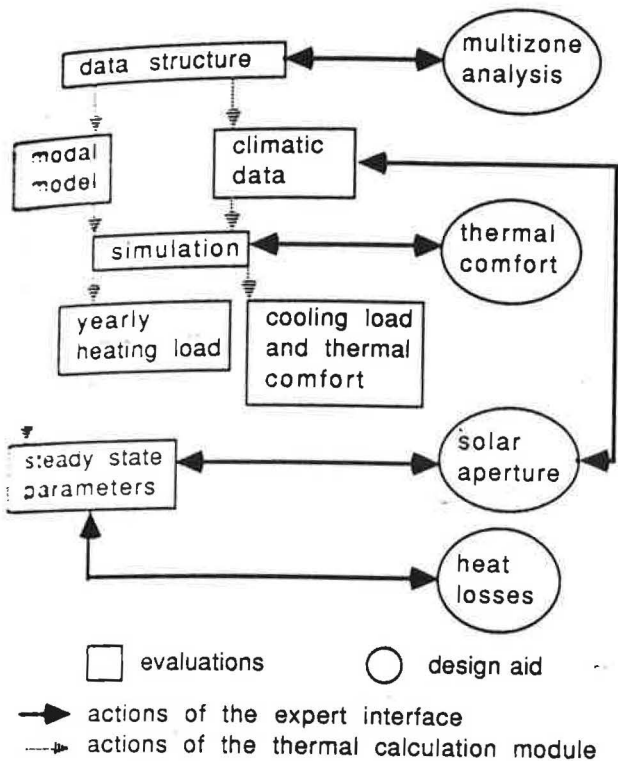
fig. 4 : structure of the software
