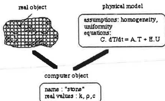
fig. 1 : example of an elementary object, the stone
