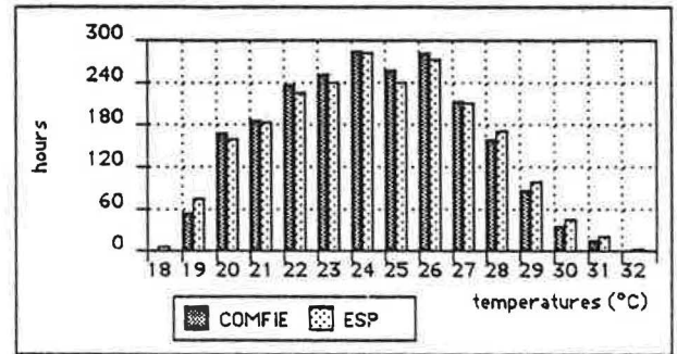
fig. 6. Temperature histograms, COMFIE versus ESP
