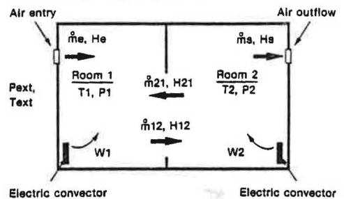
Figure 7 - Ventilation in a two room building.
