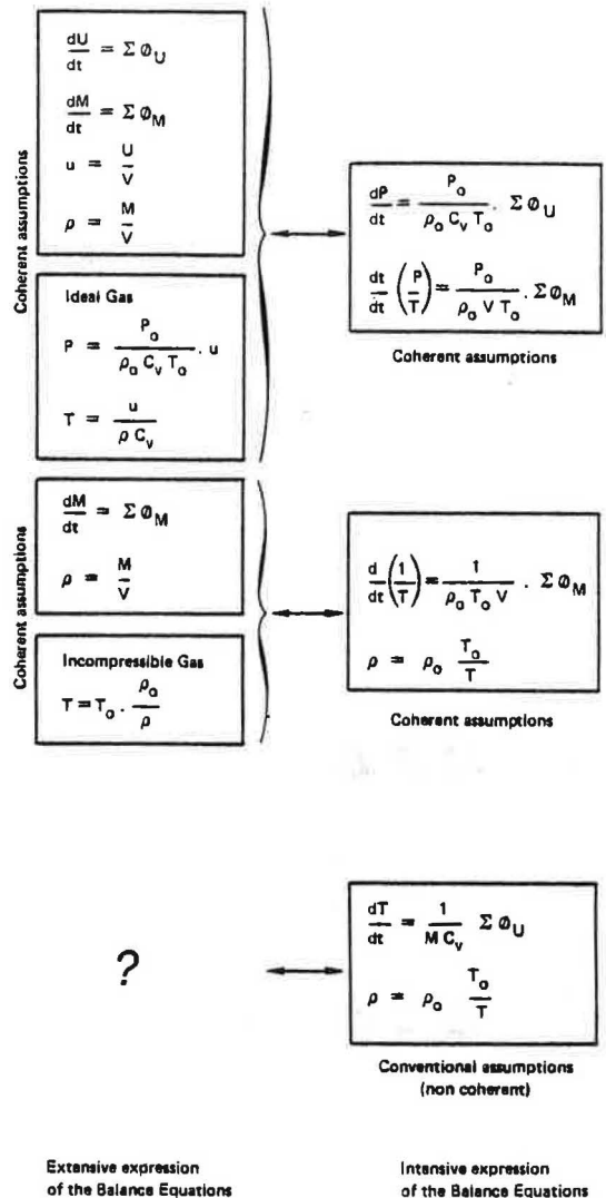
Figure 9 - Comparison between two air balance equation formulations.
