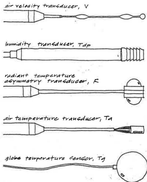
Figure 2 Transducer profiles
