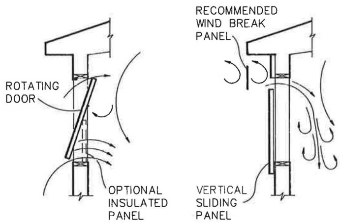
FIGURE 1 TWO COMMON METHODS OF ADJUSTING WALL OPENING SIZE. AIRFLOW PATTERNS SHOWN ARE FOR WINTER CONDITIONS
