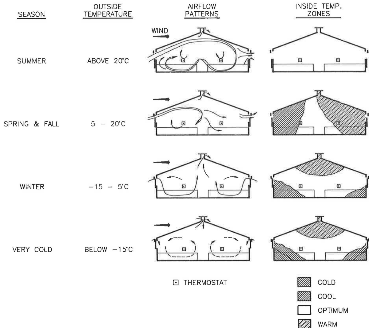
FIGURE 3 SEASONAL CHANGES IN AIRFLOW PATTERNS AND TEMPERATURE DISTRIBUTIONS IN THE ANIMAL ROOM
