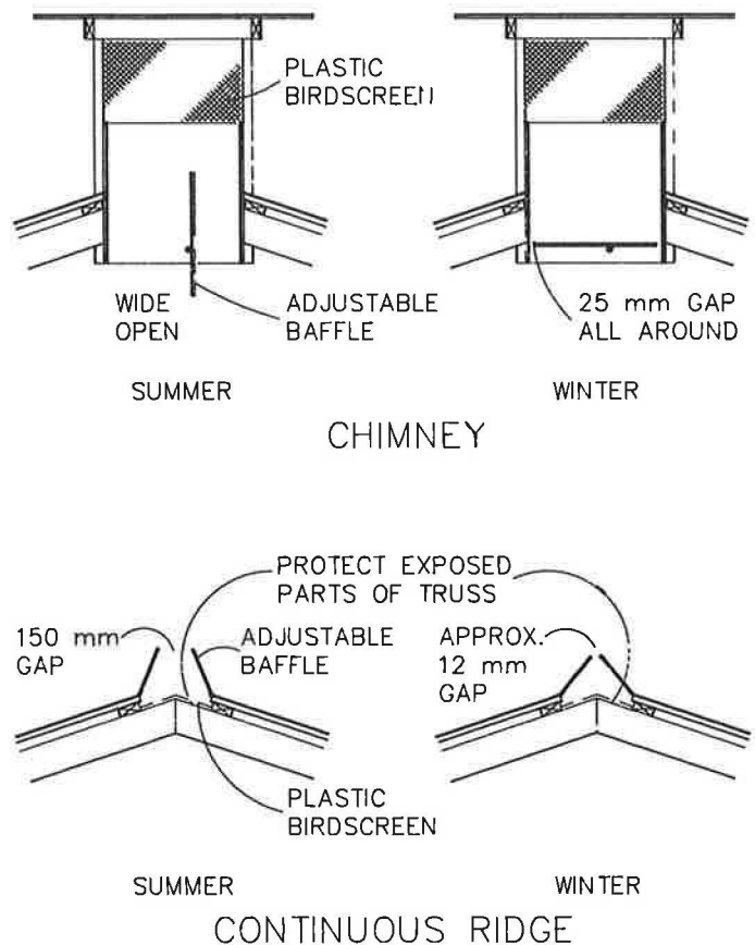
FIGURE 2 A MINIMUM RIDGE OPENING CAN BE ACHIEVED USING EITHER CHIMNEYS OR A CONTINUOUS RIDGE SLOT
