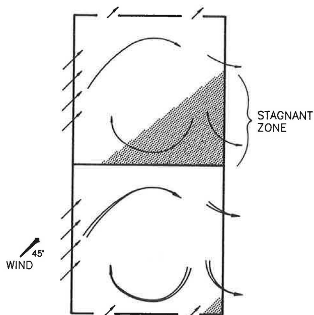
FIGURE 8 IN A MULTI-ROOM BUILDING, THE UPWIND ROOM HAS A SLIGHTLY HIGHER VENTILATION RATE
