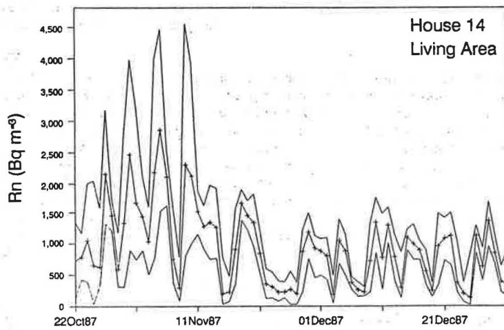
Fig. 1. Measurements of ^{222}\text{Rn} during fall in two Huntsville houses; the upper and lower curves represent daily maximum 30-minute integrated measurement while the middle curve shows the daily average ^{222}\text{Rn} concentration.
