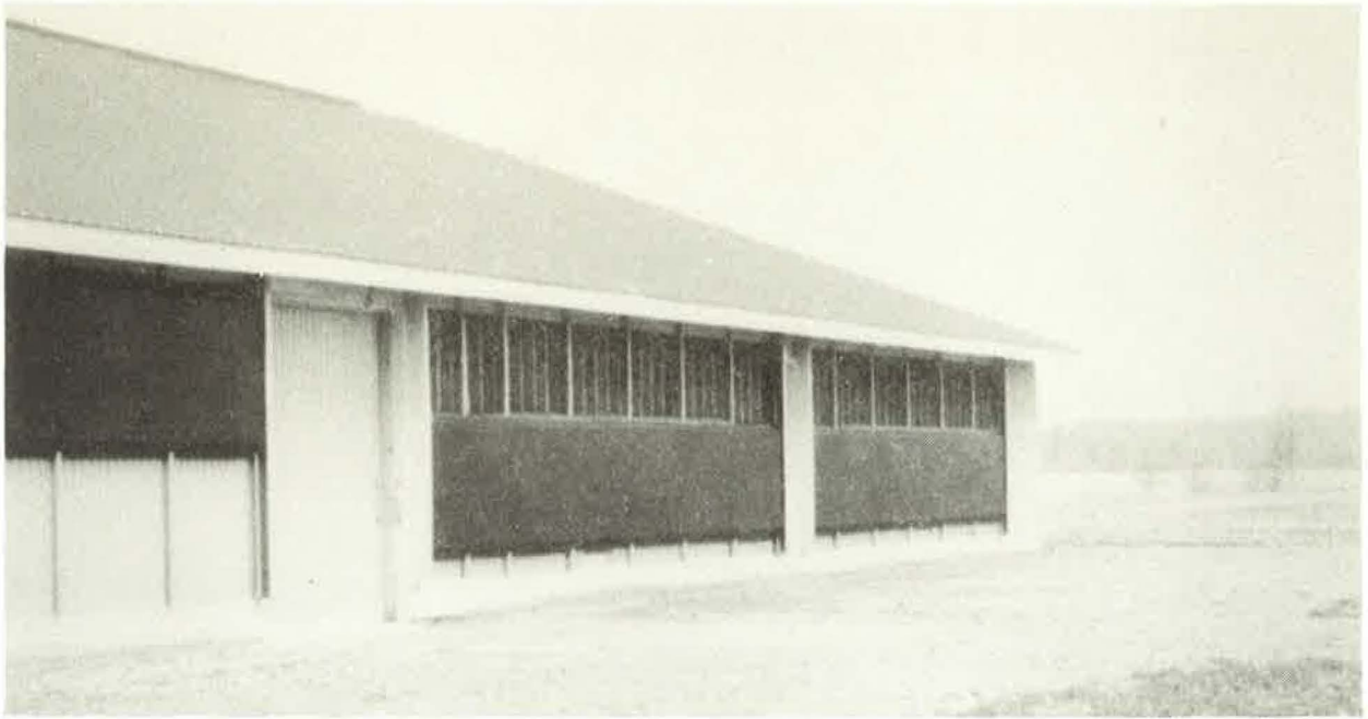
Photo 3 Insulated vertical panels are shown in both the open and closed positions on a turkey barn.
