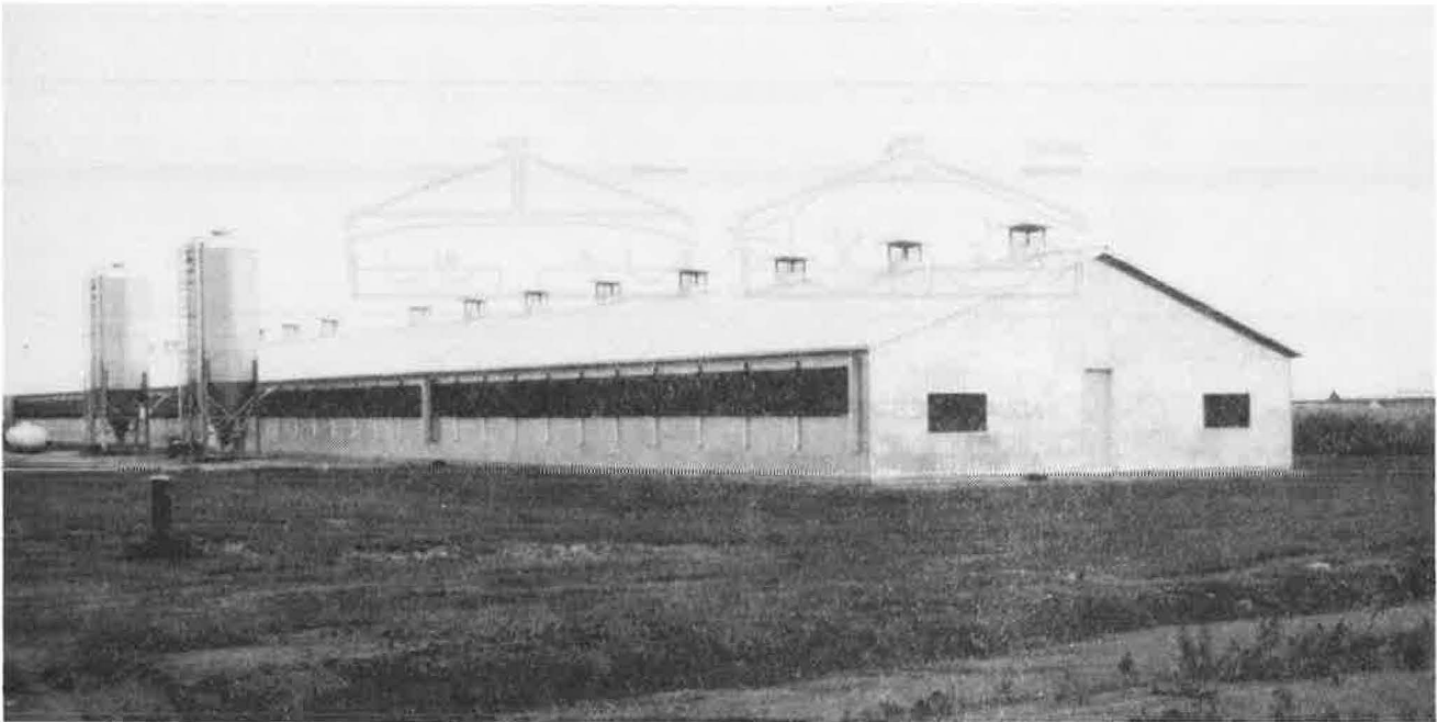
Photo 1 An automatically controlled, warm, naturally ventilated hog barn using vertically sliding sidewall panels, chimneys, and manually operated endwall openings.
