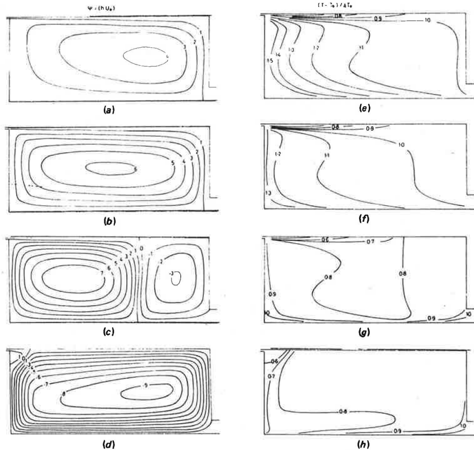
Fig. 2 Patterns of streamlines (a-d) and isotherms (e-h) at Re = 7350, L/H = 3.0, h/H = 0.017, and Ar as follows: (a and e) 0, (b and f) 8 \times 10^{-3} , (c and g) 2 \times 10^{-2} , and (d and h) 8 \times 10^{-2} .
