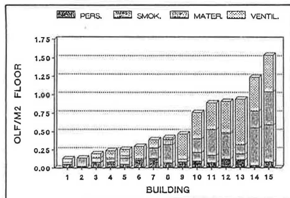
Figure 7 : Air pollution by various sources for 15 office buildings in Copenhagen /11/
