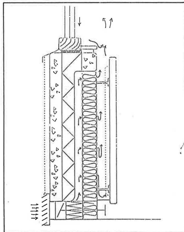
Figure 11 : Wall components also functioning as air inlet aiming to eliminate draught problems /23/
