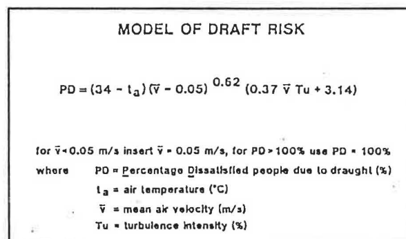
Figure 8 : Formula for estimating draught risk /13/
