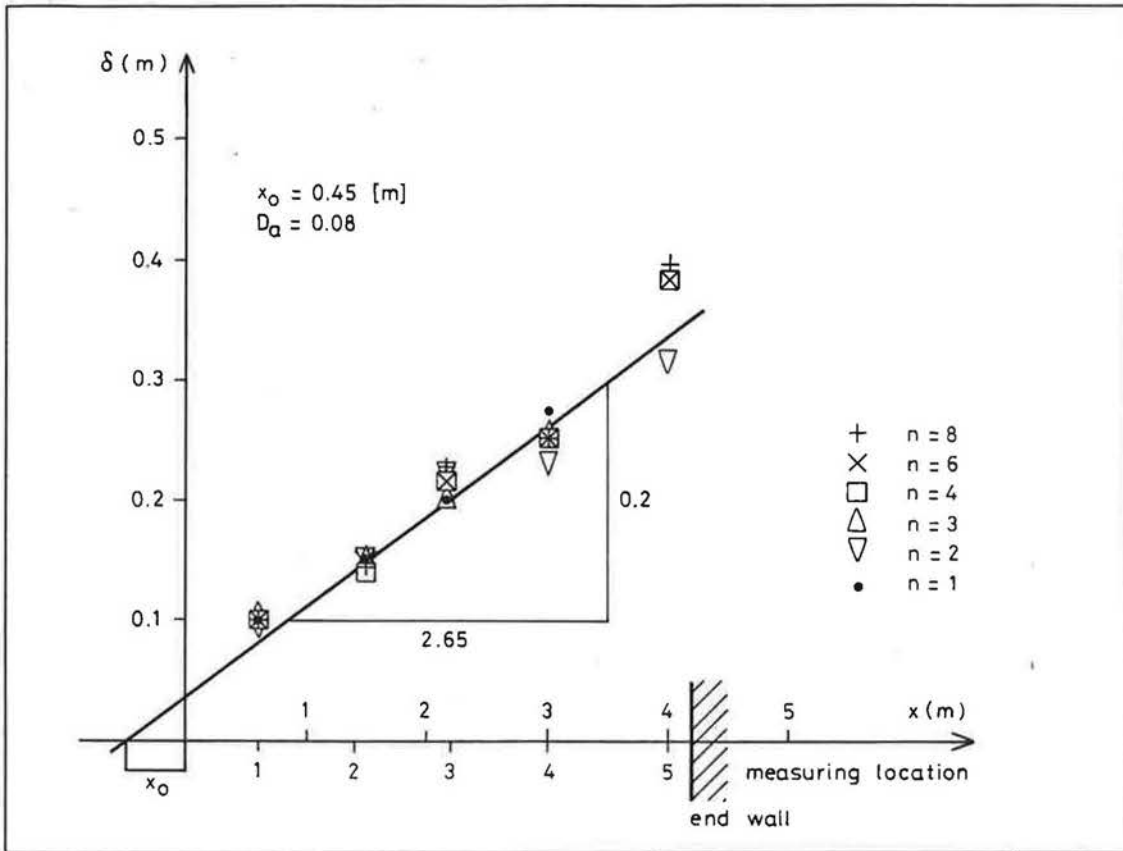
Fig. 6 : The width \delta in the xy - plane as a function of x . D_a is found to be 0.08 and x_0 is found to be 0.45m.
