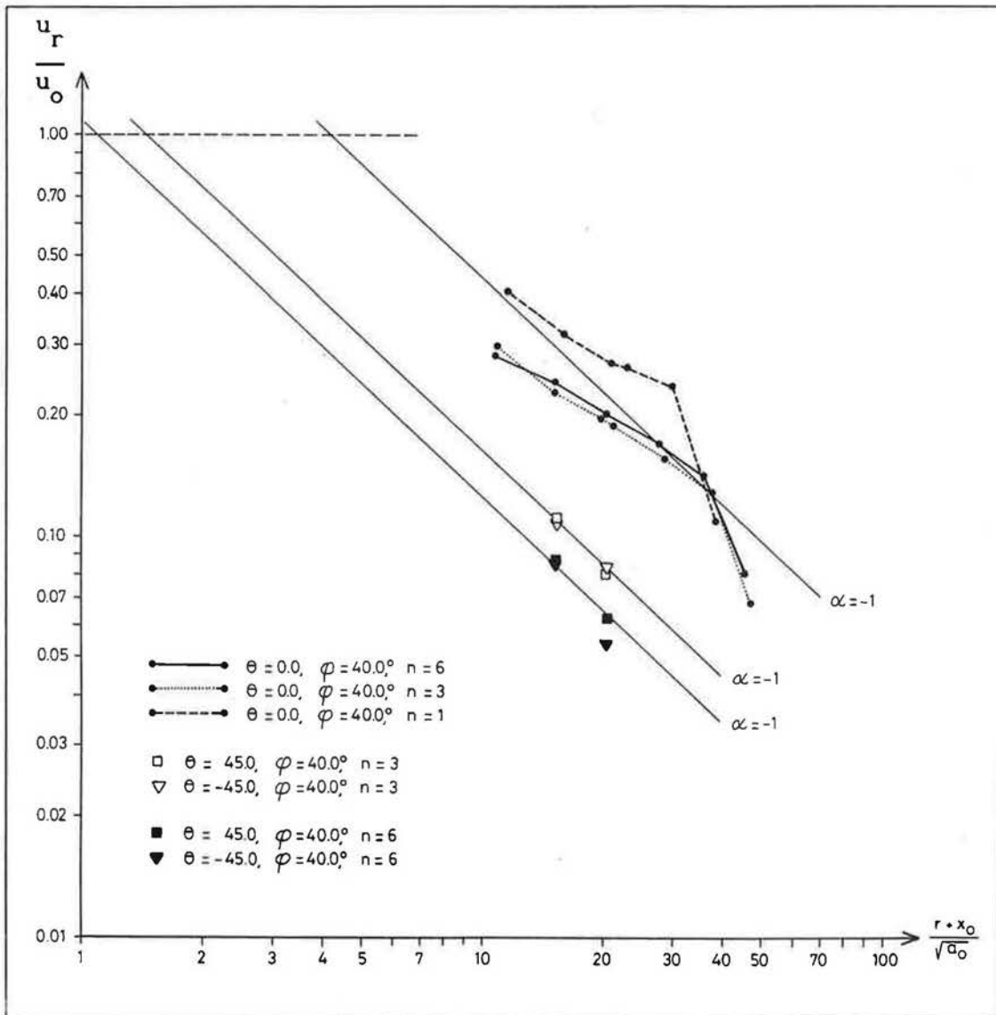
Fig. 10 : The decay of the maximum velocity for different air change rates at different \vartheta values. The K(40,0) is found to 4.2 and the k(40, \pm 45) is found to 1.1-1.5.
