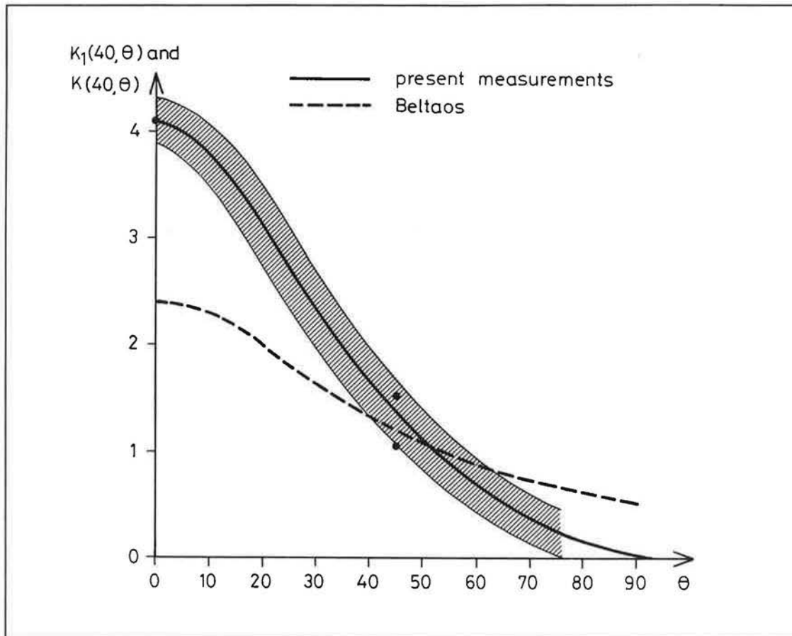
Fig 11 : Comparison of the K(40, \vartheta) values found in a circular impinging jet an in the inlet flow from a HESCO -diffuser.
