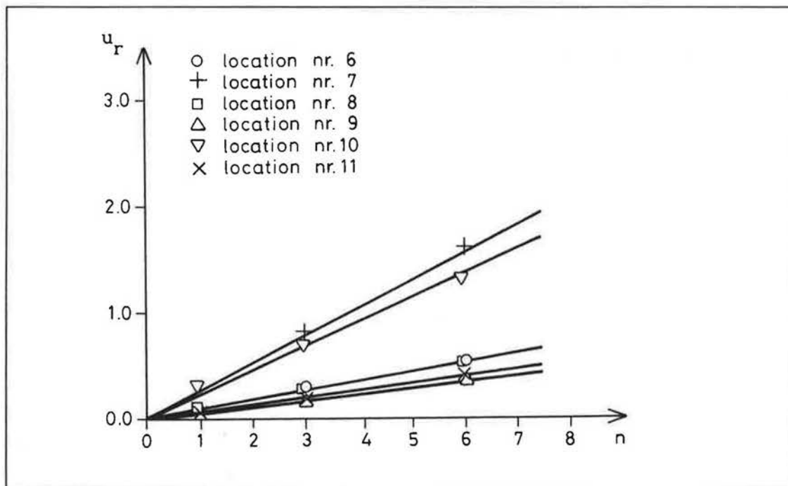
Fig. 9 : The maximum velocities at \theta = 0^\circ and \pm 45^\circ as functions of the air change rate. \phi = 40^\circ .
