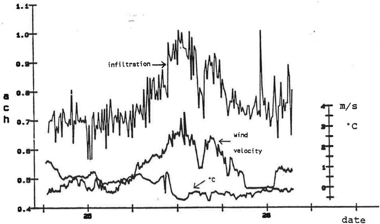
Figure 3.2.1. The influence of the wind velocity on the infiltration rate (the whole house). Inlets and outlets were shut and the occupants came home late in the evening the 25th.
