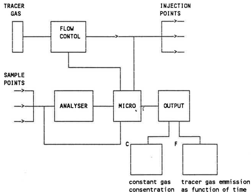
Figure 2.1. Schematic of constant concentration equipment
