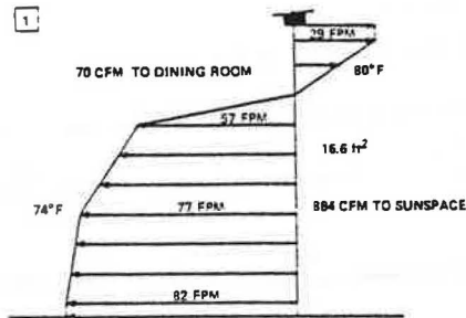
Fig. 4. Corrected velocity profile in aperture 1, located between the dining room and the sunspace.
