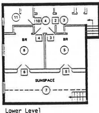
Fig. 3. Floor plans of La Vereda, Model 4. The west end is two story; and the east, entry end is single story at an intermediate level. Arrows on stairs show traffic down. Circles refer to room numbers, and squares refer to aperture numbers.
