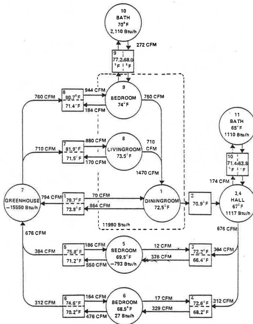
Fig. 6. Natural airflow diagram in La Vereda, Model 4, at 2:00 p.m., January 11, 1983, a sunny day. See Fig. 3 for identification numbers of rooms (circles) and apertures (squares). Airflow rates and velocity-weighted average temperatures are shown for each airflow direction for each aperture. Net energy flow rates are shown for the rooms, but note that rooms 1, 8, and 9 cannot be disaggregated so that the total energy deposited in the three rooms (11980 Btu/h) refers to the region enclosed by the dotted line. Room temperatures shown are \pm 1^\circ\text{F} . Greenhouse temperatures ranged from 68^\circ\text{F} near the floor to 82^\circ\text{F} near the ceiling.
