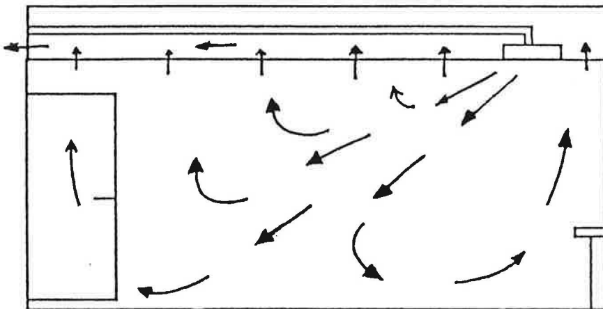
Fig. 4: Typical air flow pattern determined by smoke visualization System type: Complete mixing / ceiling outlet
