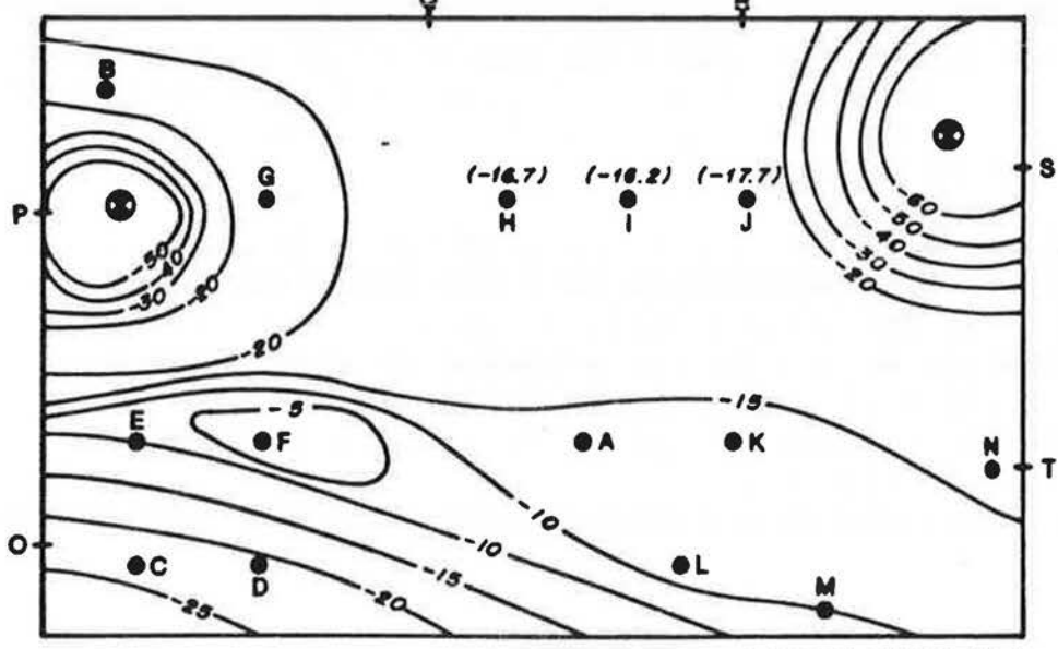
PRESSURE CONTOURS WITH REDUCED SUCTION (MAY 8)
