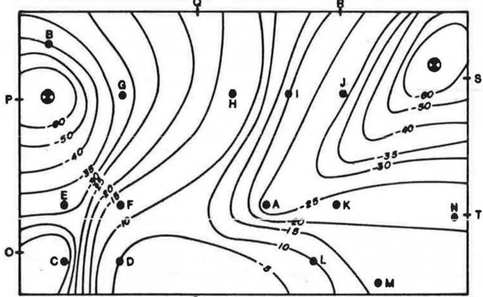
PRESSURE CONTOURS WITH TWO VAPOUR WELLS (MAY 2)
