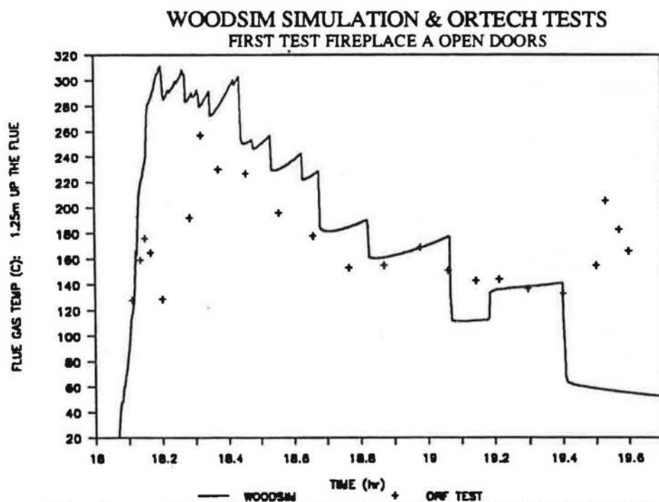
FIGURE 7. FIRST COMPARISON BETWEEN WOODSIM SIMULATION & ORTECH TEST FLUE GAS AND FLUE LINER TEMPERATURES
