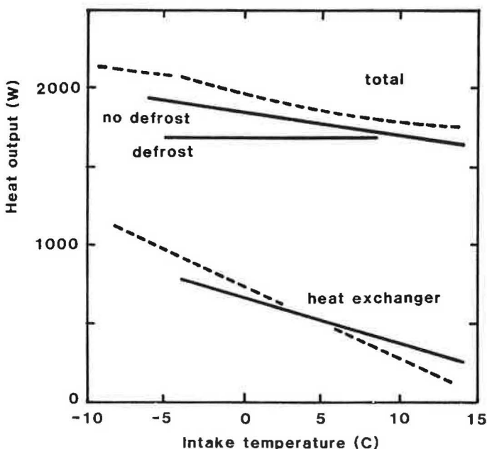
Figure 5 Heat output of unit as a function of intake temperature, normalised to a house extract temperature of 20^{\circ}\text{C} and a flow rate of 180 \text{ m}^3 \text{ h}^{-1} . Broken curve manufacturer's data, full curve measurements.
