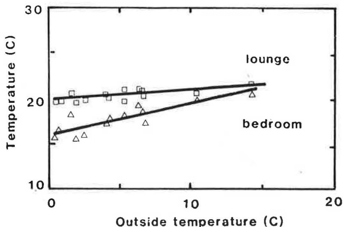
Figure 7 Weekly average room temperatures as a function of outside temperature
