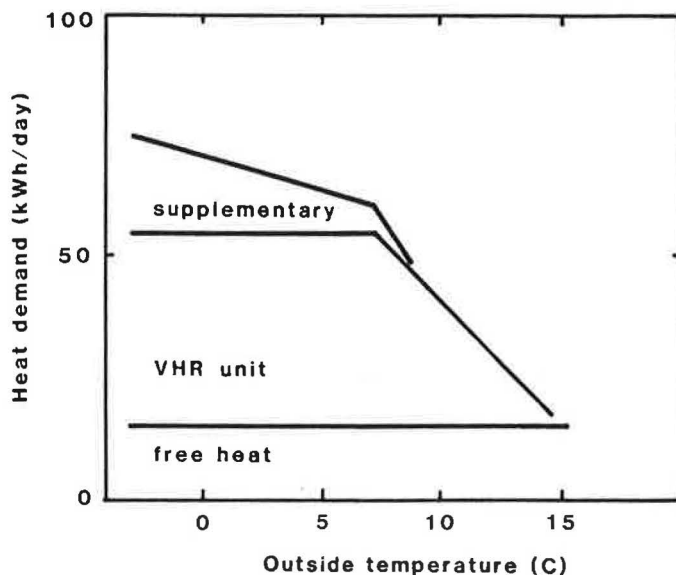
Figure 8 Heat supplied to the house per day as a function of outside air temperature. This is a smoothed version of the actual daily consumptions, and is not corrected for variations in internal temperature.
