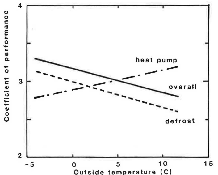
Figure 6 Coefficient of performance of the unit as a function of intake temperature, normalised to a house temperature of 20^{\circ}\text{C} and a flow rate of 180 \text{ m}^3 \text{ h}^{-1} . COP is shown for the heat pump alone, and for the overall system, both with and without the effects of defrost operation.
