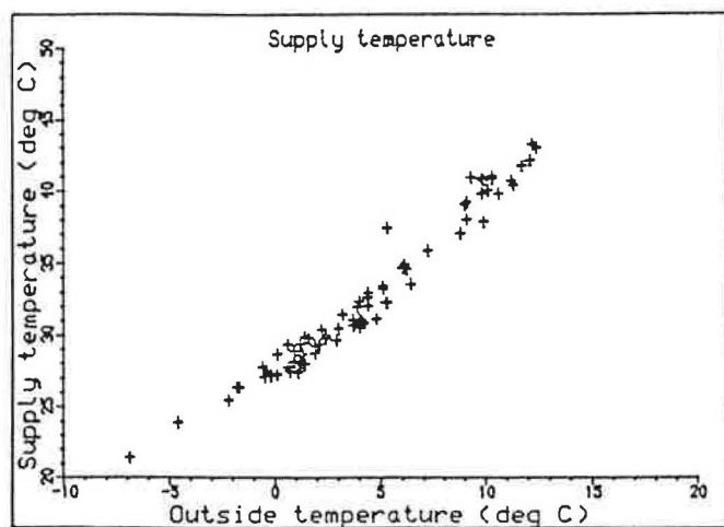
Figure 3 Supply temperature as a function of outside temperature. Each point is a 24 h average, and is uncorrected for the effects of defrosting or internal temperature.
