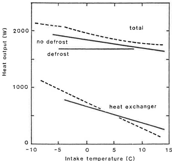
Figure 5 Heat output of unit as a function of intake temperature, normalised to a house extract temperature of 20^{\circ}\text{C} and a flow rate of 180 \text{ m}^3 \text{ h}^{-1} . Broken curve manufacturer's data, full curve measurements.
