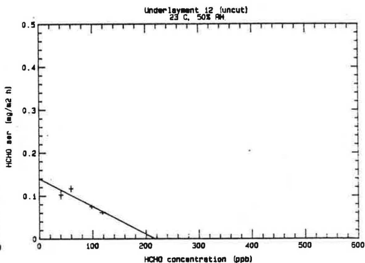
Figure 20. HCHO Emission Rate for Underlayment #12 as a Function of HCHO Concentration (first test).*
