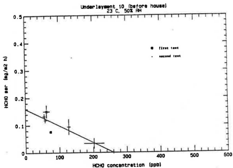
Figure 18. HCHO Emission Rate for Underlayment #10 as a Function of HCHO Concentration (first and second tests).*
