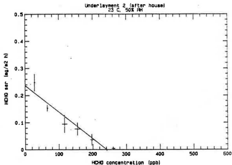
Figure 10. HCHO Emission Rate for Underlayment #2 as a Function of HCHO Concentration (third test).*
