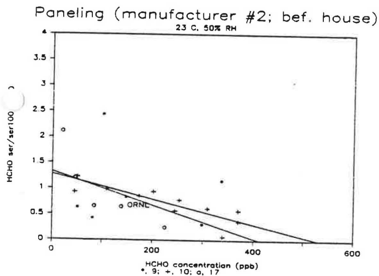
Figure 75. Comparison of Normalized HCHO Emission Rates for Combined Paneling from manufacturer #2 (before prototype house study) to those Predicted by ORNL Emission Model.
