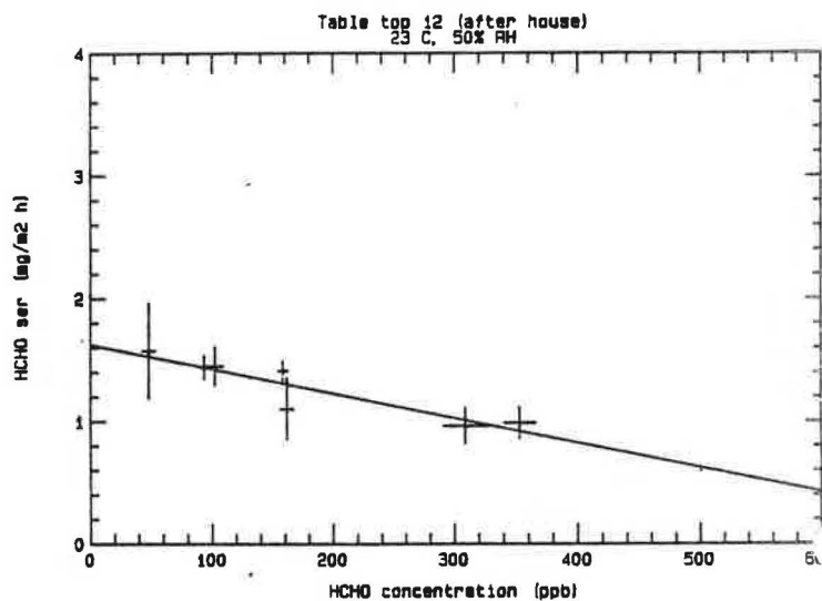
Figure 38. HCHO Emission Rate for MDF Table Top #12 as a Function of HCHO Concentration (third test.)*
