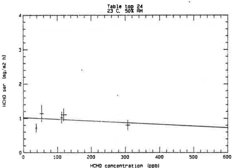
Figure 39. HCHO Emission Rate for MDF Table Top #24 as a Function of HCHO Concentration.*
