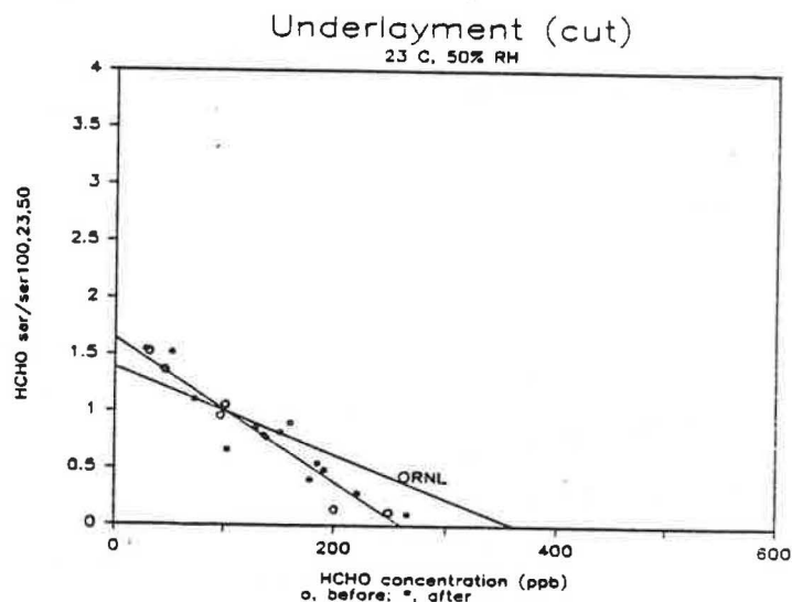
Figure 74. Comparison of Normalized HCHO Emission Rates for Combined Cut Underlayment to those Predicted by ORNL Emission Model.
