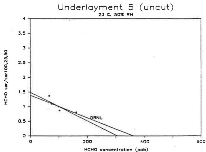
Figure 42. Comparison of Normalized HCHO Emission Rates for Underlayment #5 (first test) to those Predicted by ORNL Emission Model.
