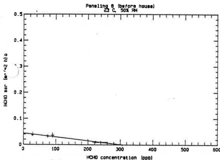
Figure 27. HCHO Emission Rate for Paneling #8 as a Function of HCHO Concentration (first test).*
