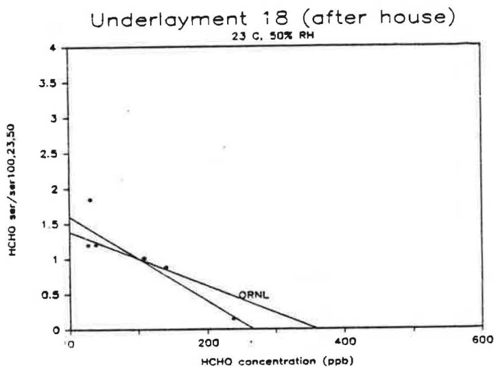
Figure 55. Comparison of Normalized HCHO Emission Rates for Underlayment #18 (second test) to those Predicted by ORNL Emission Model.
