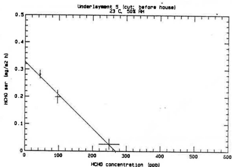
Figure 12. HCHO Emission Rate for Underlayment #5 as a Function of HCHO Concentration (second test).*
