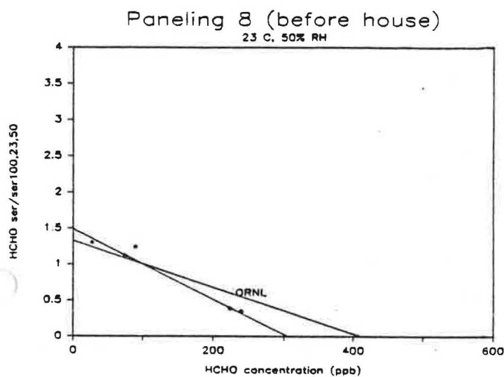
Figure 57. Comparison of Normalized HCHO Emission Rates for Paneling #8 (first test) to those Predicted by ORNL Emission Model.
