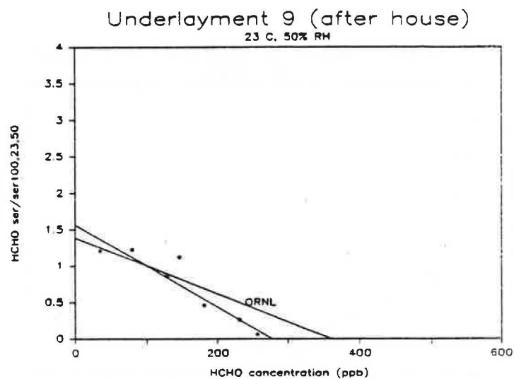
Figure 48. Comparison of Normalized HCHO Emission Rates for Underlayment #9 (third test) to those Predicted by ORNL Emission Model.
