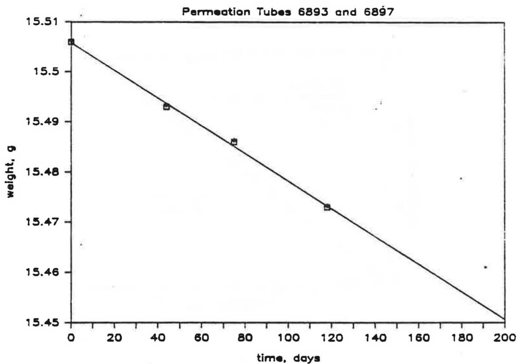
Figure 5. Weight Loss Calibration for Permeation Tubes used for Calibrating HCHO Monitor.
