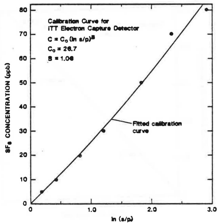
Figure 8. Calibration Curve for ITT Electron-Capture Gas Chromatograph (Medium-Size Chambers).
