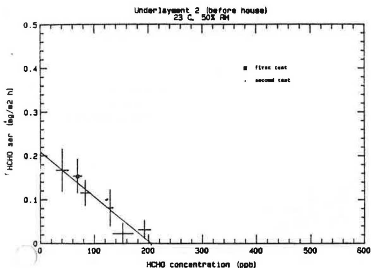
Figure 9. HCHO Emission Rate for Underlayment #2 as a Function of HCHO Concentration (first and second tests).*
