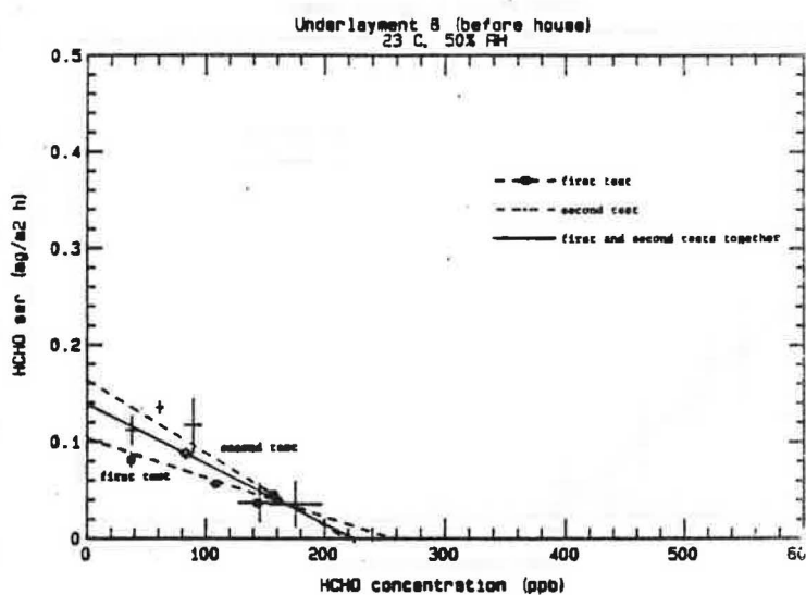
Figure 14. HCHO Emission Rate for Underlayment #8 as a Function of HCHO Concentration (first and second tests).*
