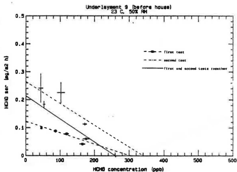
Figure 16. HCHO Emission Rate for Underlayment #9 as a Function of HCHO Concentration (first and second tests).*
