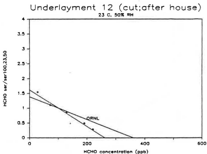
Figure 53. Comparison of Normalized HCHO Emission Rates for Underlayment #12 (third test) to those Predicted by ORNL Emission Model.
