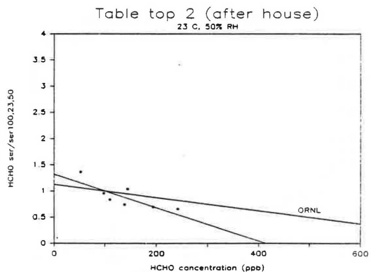
Figure 64. Comparison of Normalized HCHO Emission Rates for MDF Table Top #2 (third test) to those Predicted by ORNL Emission Model.
