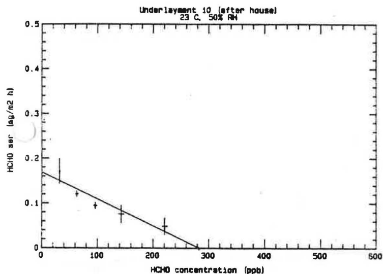
Figure 19. HCHO Emission Rate for Underlayment #10 as a Function of HCHO Concentration (third test).*
