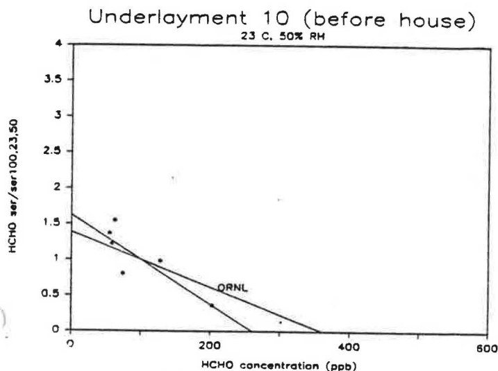
Figure 49. Comparison of Normalized HCHO Emission Rates for Underlayment #10 (first and second tests combined) to those Predicted by ORNL Emission Model.
