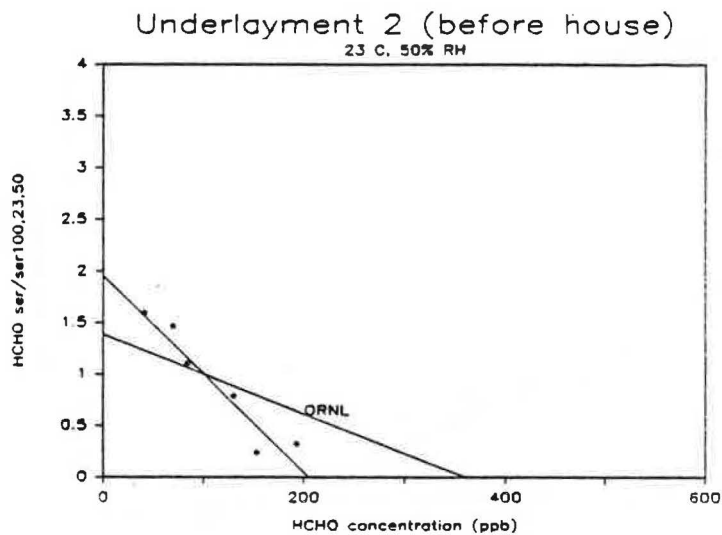
Figure 40. Comparison of Normalized HCHO Emission Rates for Underlayment #2 (first and second tests combined) to those Predicted by ORNL Emission Model.
