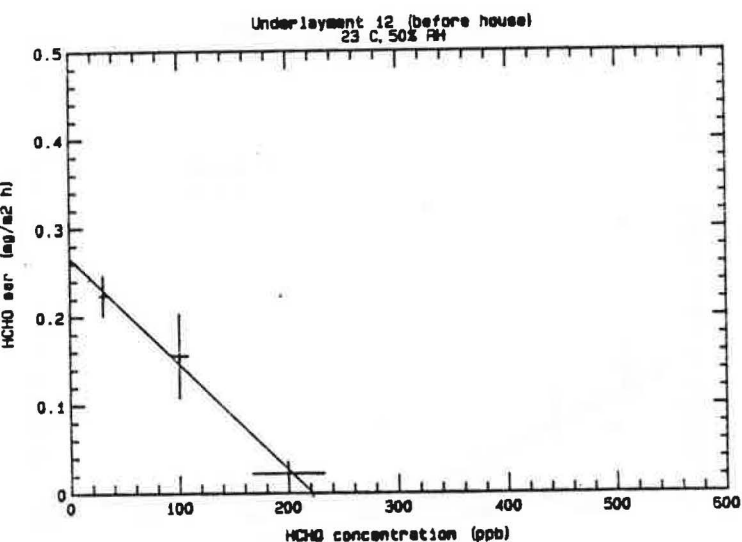
Figure 21. HCHO Emission Rate for Underlayment #12 as a Function of HCHO Concentration (second test).*
