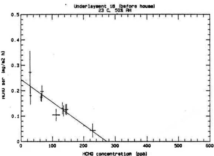
Figure 23. HCHO Emission Rate for Underlayment #18 as a Function of HCHO Concentration (first test).*
