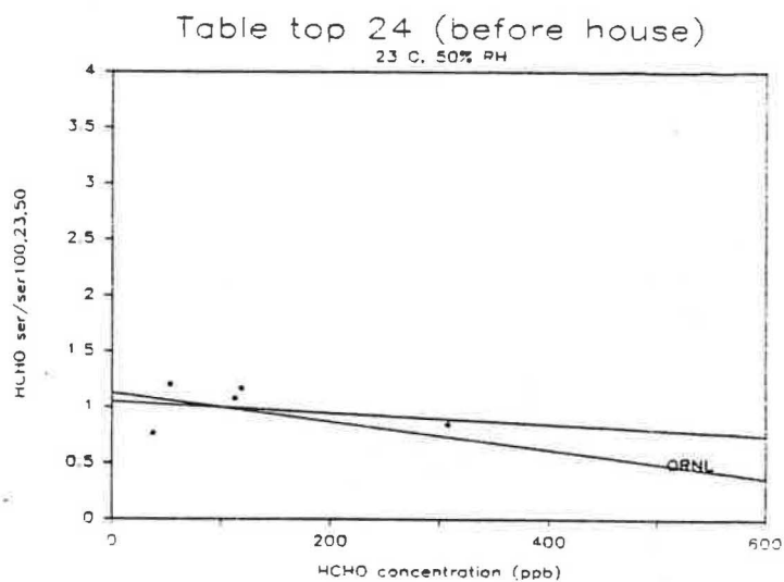
Figure 68. Comparison of Normalized HCHO Emission Rates for MDF Table Top #24 to those Predicted by ORNL Emission Model.
