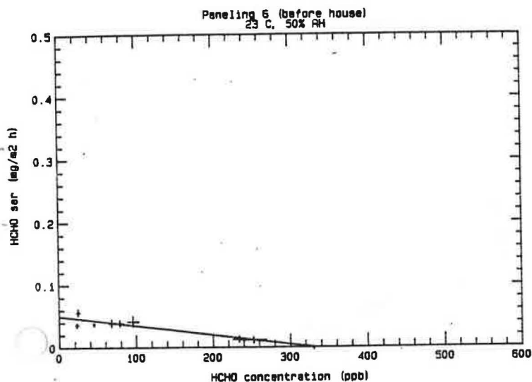
Figure 25. HCHO Emission Rate for Paneling #6 as a Function of HCHO Concentration (first test).*
