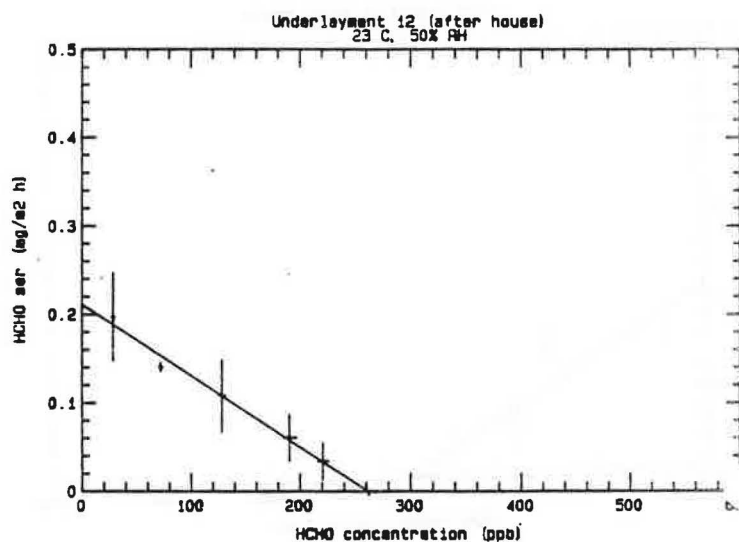
Figure 22. HCHO Emission Rate for Underlayment #12 as a Function of HCHO Concentration (third test).*
