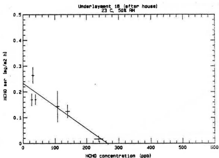
Figure 24. HCHO Emission Rate for Underlayment #18 as a Function of HCHO Concentration (second test).*
