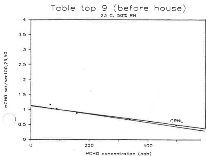
Figure 65. Comparison of Normalized HCHO Emission Rates for MDF Table Top #9 to those Predicted by ORNL Emission Model.
