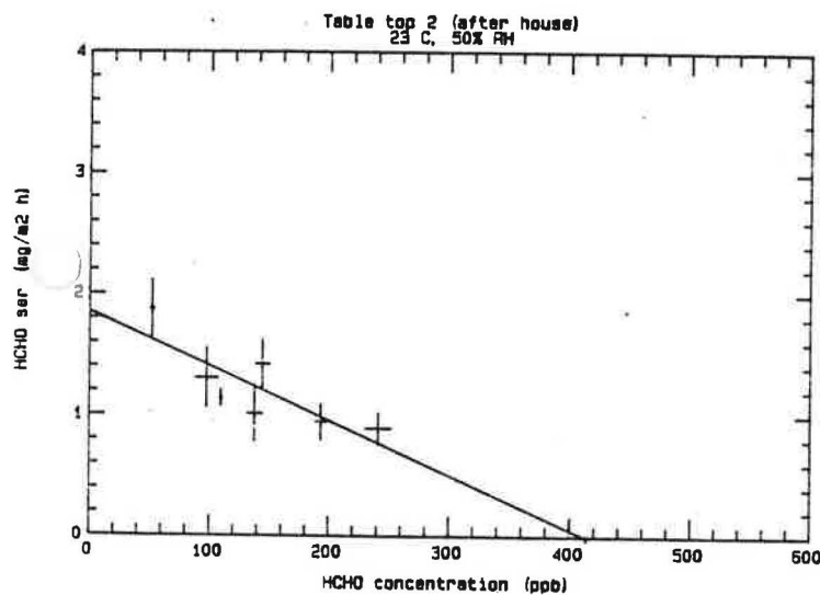
Figure 35. HCHO Emission Rate for MDF Table Top #2 as a Function of HCHO Concentration (third test.)*
