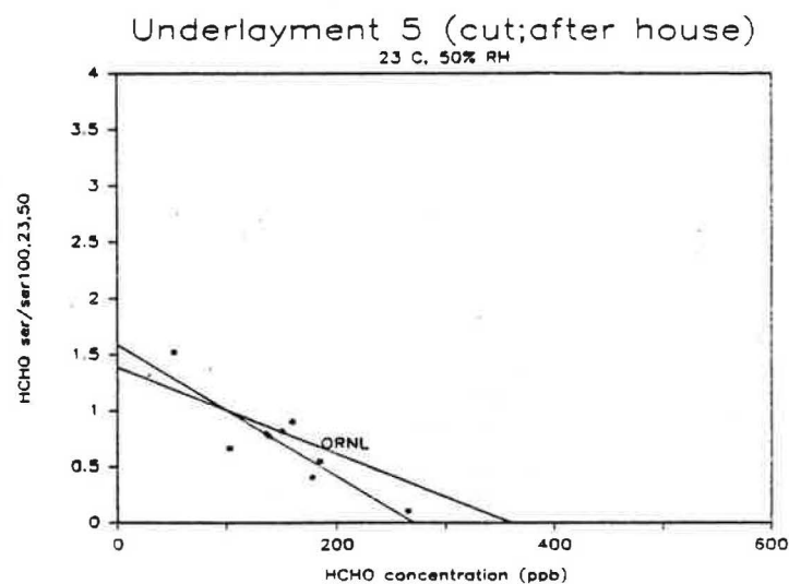
Figure 44. Comparison of Normalized HCHO Emission Rates for Underlayment #5 (third test) to those Predicted by ORNL Emission Model.
