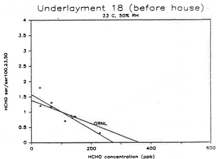
Figure 54. Comparison of Normalized HCHO Emission Rates for Underlayment #18 (first test) to those Predicted by ORNL Emission Model.
