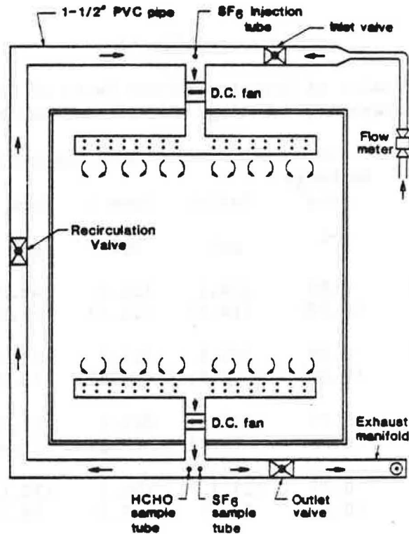
Figure 1. Schematic of Medium-Size Chamber for Measuring HCHO Emission Rates.
