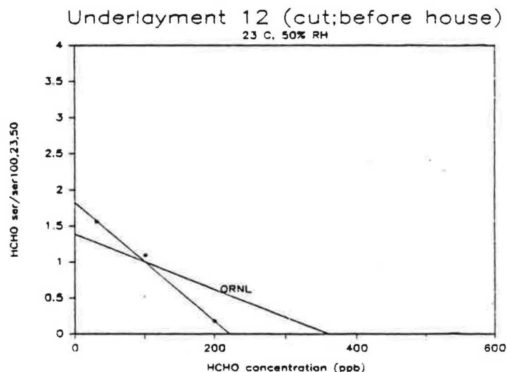
Figure 52. Comparison of Normalized HCHO Emission Rates for Underlayment #12 (second test) to those Predicted by ORNL Emission Model.
