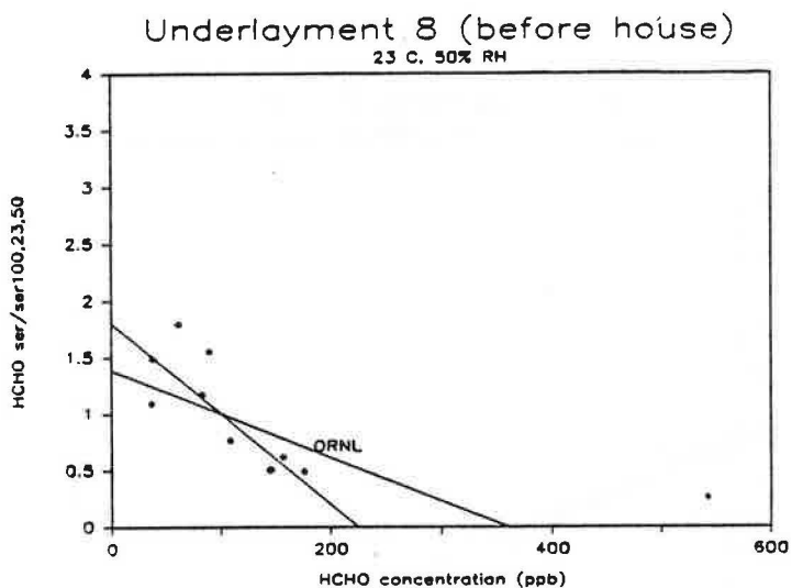
Figure 45. Comparison of Normalized HCHO Emission Rates for Underlayment #8 (first and second tests combined) to those Predicted by ORNL Emission Model.
