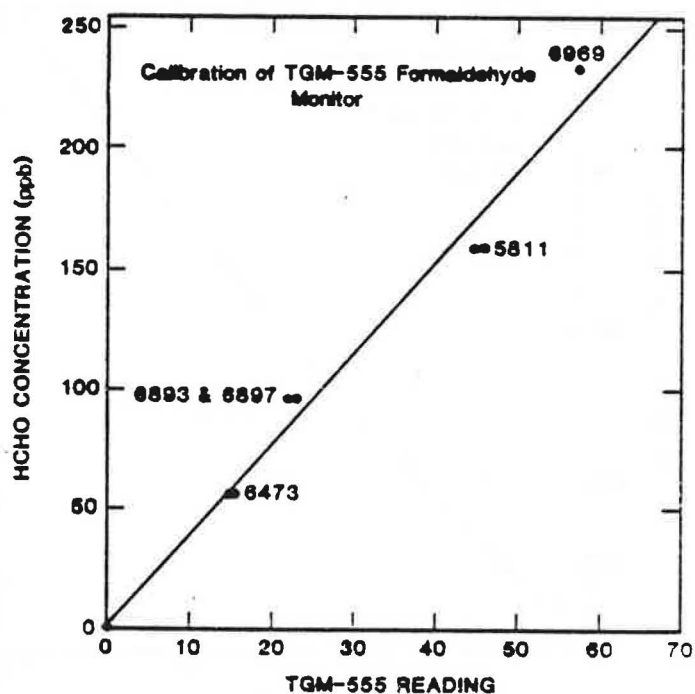
Figure 6. Calibration Curve of the HCHO Concentration Monitor. (The numbers alongside the line are identifying numbers for permeation tubes.)
