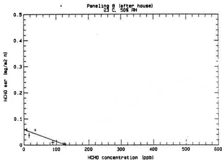
Figure 28. HCHO Emission Rate for Paneling #8 as a Function of HCHO Concentration (second test).*
