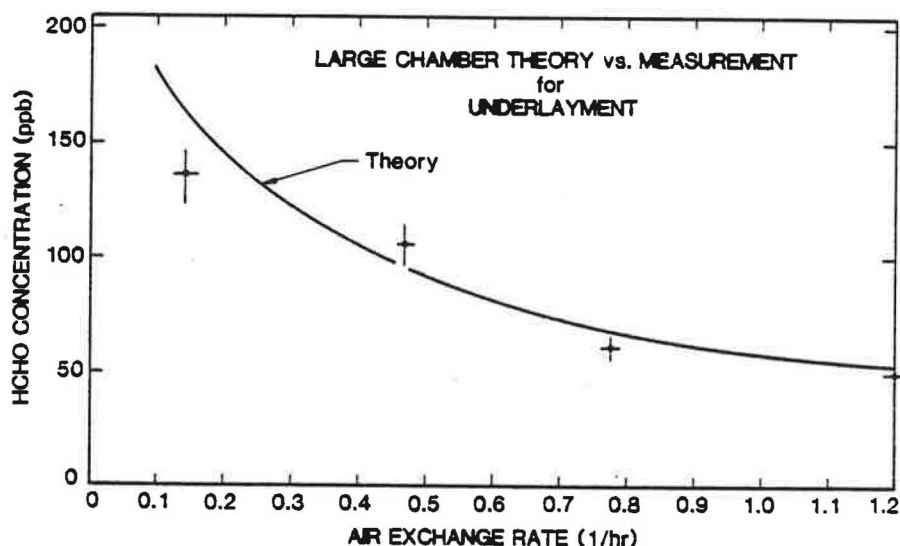
Figure 80. Comparison of Measurements (points) and Predictions of Equation 8 (curve) for Prototype-House Loading of Underlayment.*
