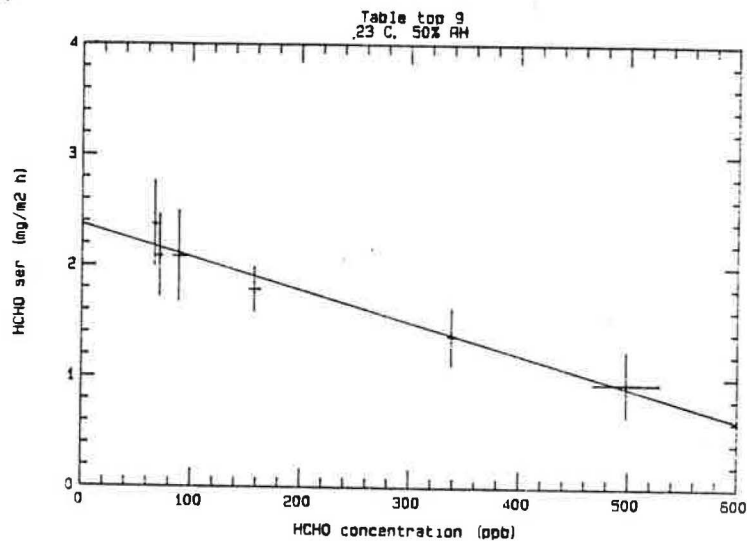
Figure 36. HCHO Emission Rate for MDF Table Top #9 as a Function of HCHO Concentration.*
