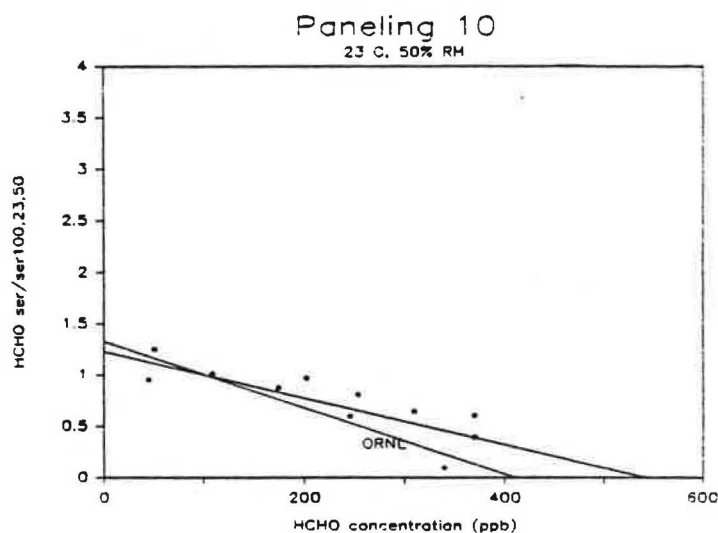
Figure 60. Comparison of Normalized HCHO Emission Rates for Paneling #10 to those Predicted by ORNL Emission Model.
