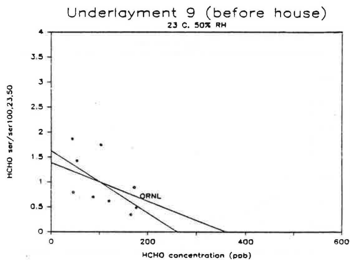
Figure 47. Comparison of Normalized HCHO Emission Rates for Underlayment #9 (first and second tests combined) to those Predicted by ORNL Emission Model.
