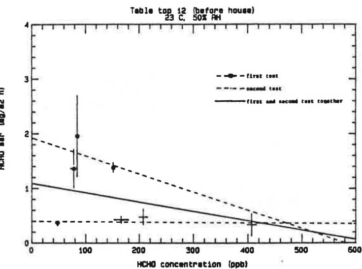
Figure 37. HCHO Emission Rate for MDF Table Top #12 as a Function of HCHO Concentration (first and second tests.)*
