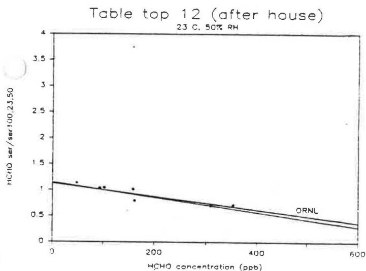
Figure 67. Comparison of Normalized HCHO Emission Rates for MDF Table Top #12 (third test) to those Predicted by ORNL Emission Model.
