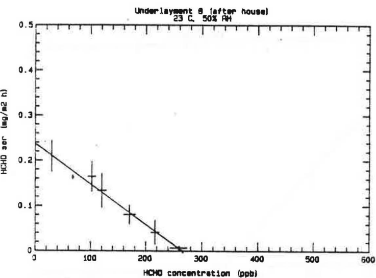
Figure 15. HCHO Emission Rate for Underlayment #8 as a Function of HCHO Concentration (third test).*
