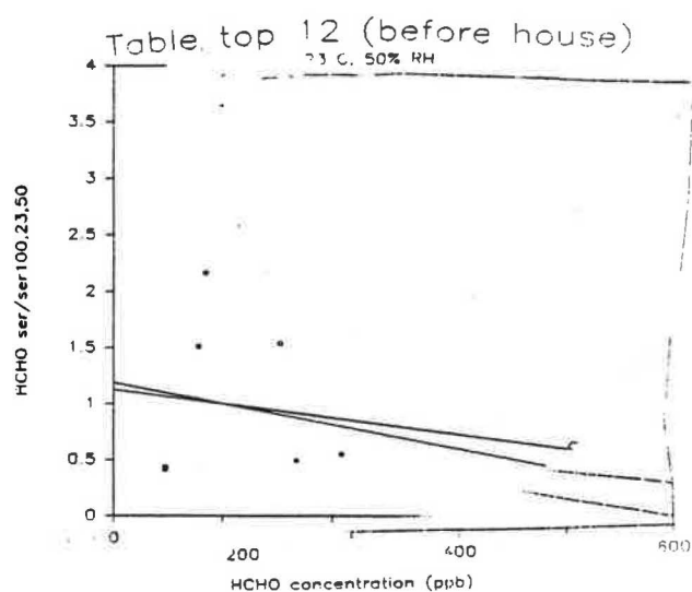
Figure 66. Comparison of Normalized HCHO Emission Rates for MDF Table Top #12 (first and second tests combined) to those Predicted by ORNL Emission Model.
