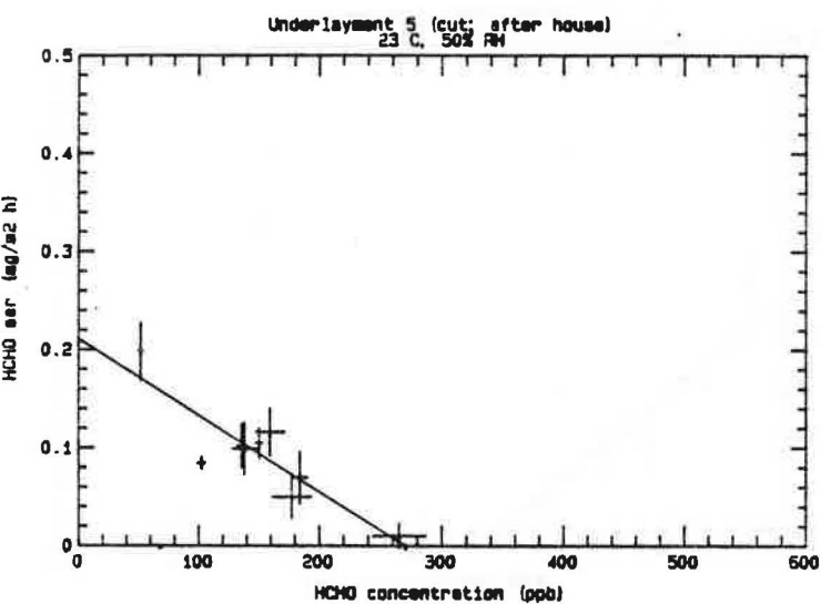
Figure 13. HCHO Emission Rate for Underlayment #5 as a Function of HCHO Concentration (third test).*
