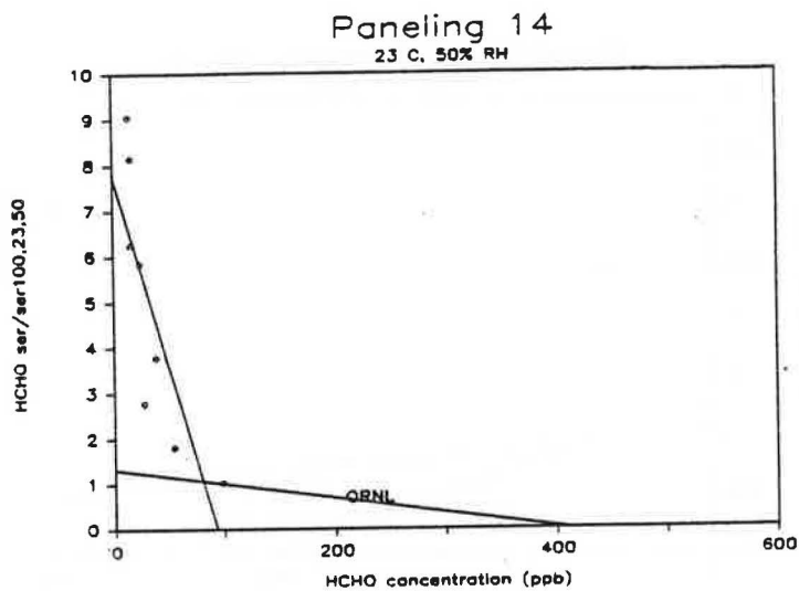
Figure 61. Comparison of Normalized HCHO Emission Rates for Paneling #14 to those Predicted by ORNL Emission Model.
