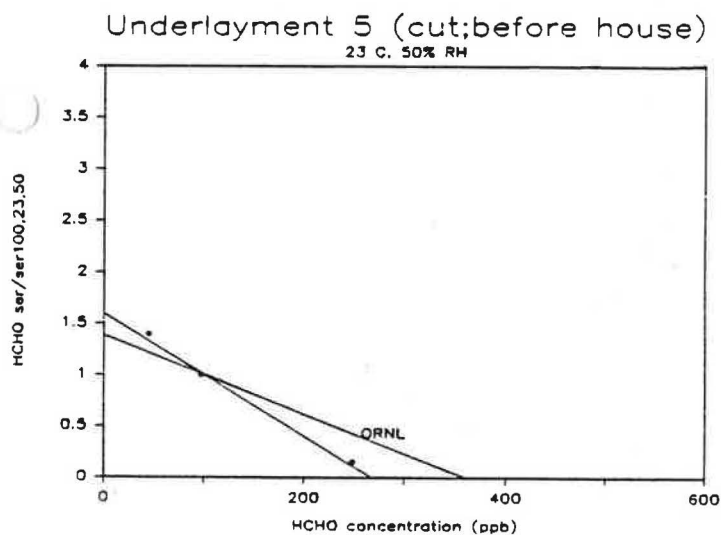
Figure 43. Comparison of Normalized HCHO Emission Rates for Underlayment #5 (second test) to those Predicted by ORNL Emission Model.
