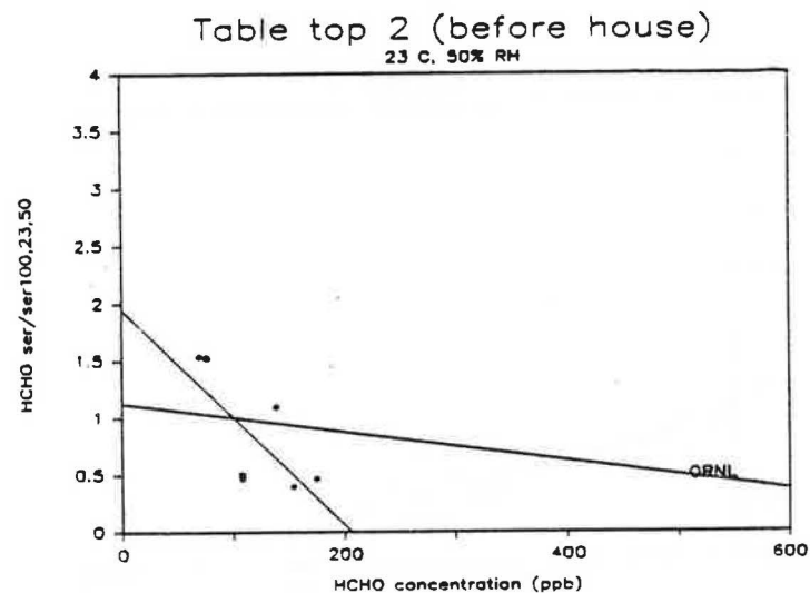
Figure 63. Comparison of Normalized HCHO Emission Rates for MDF Table Top #2 (first and second tests combined) to those Predicted by ORNL Emission Model.
