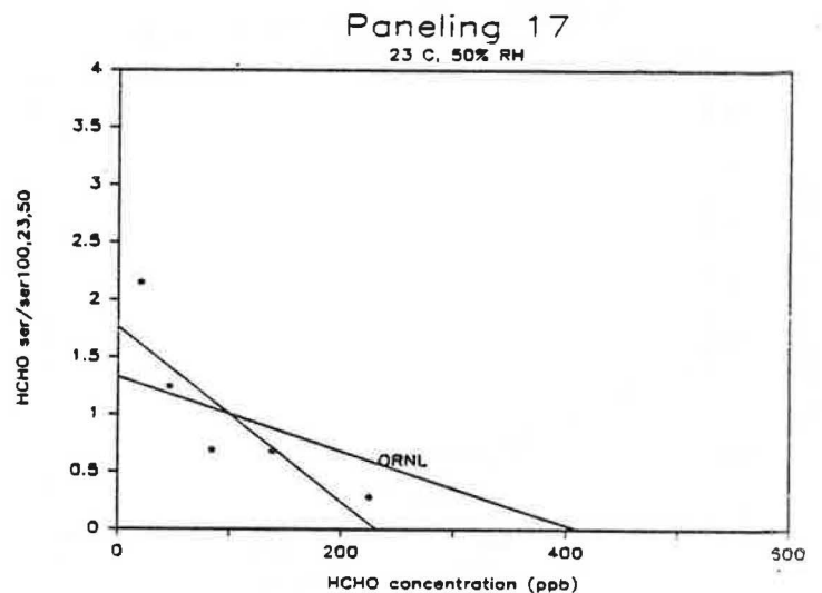
Figure 62. Comparison of Normalized HCHO Emission Rates for Paneling #17 to those Predicted by ORNL Emission Model.
