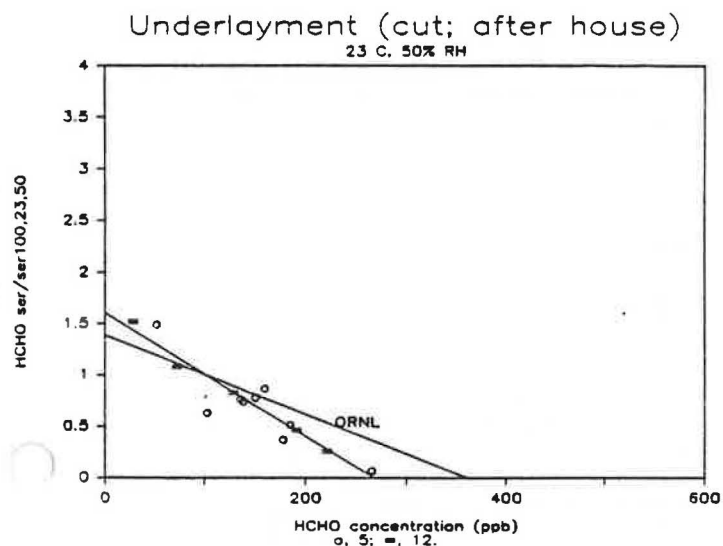
Figure 73. Comparison of Normalized HCHO Emission Rates for Combined Cut Underlayment (after prototype house study) to those Predicted by ORNL Emission Model.
