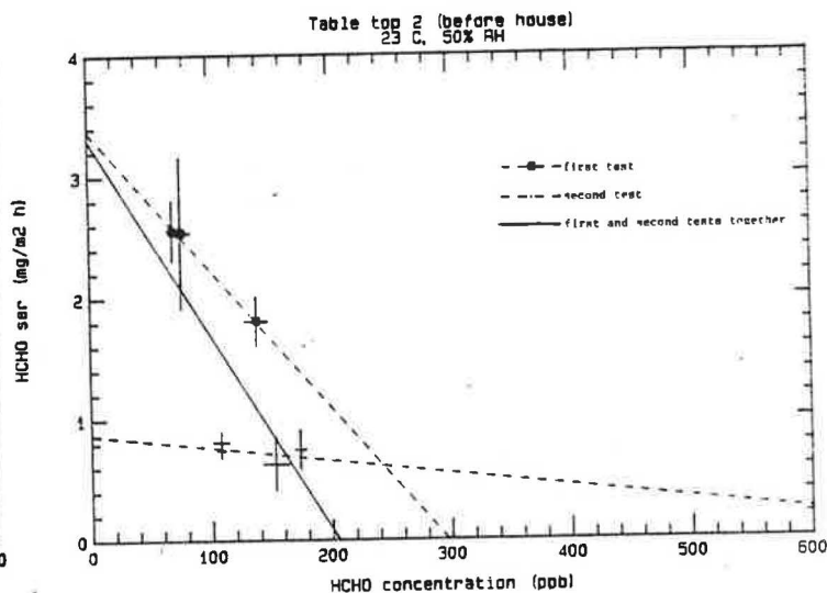
Figure 34. HCHO Emission Rate for MDF Table Top #2 as a Function of HCHO Concentration (first and second tests.)*
