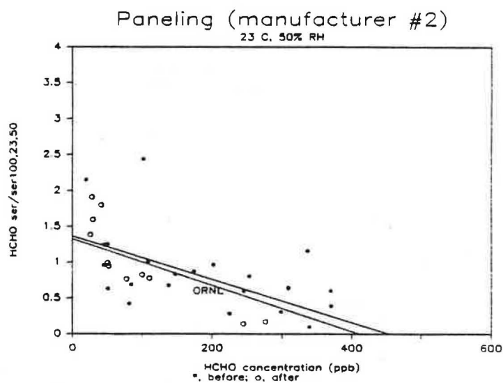
Figure 76. Comparison of Normalized HCHO Emission Rates for Combined Paneling from manufacturer #2 to those Predicted by ORNL Emission Model.
