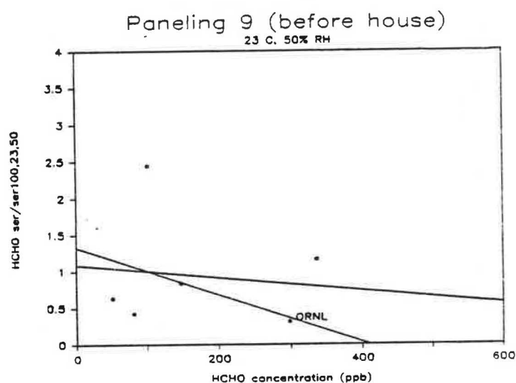
Figure 58. Comparison of Normalized HCHO Emission Rates for Paneling #9 (first test) to those Predicted by ORNL Emission Model.
