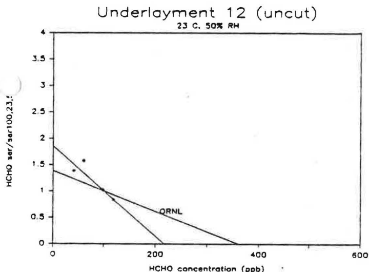
Figure 51. Comparison of Normalized HCHO Emission Rates for Underlayment #12 (first test) to those Predicted by ORNL Emission Model.
