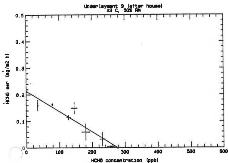
Figure 17. HCHO Emission Rate for Underlayment #9 as a Function of HCHO Concentration (third test).*
