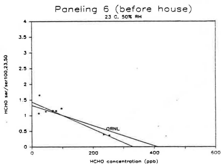
Figure 56. Comparison of Normalized HCHO Emission Rates for Paneling #6 (first test) to those Predicted by ORNL Emission Model.
