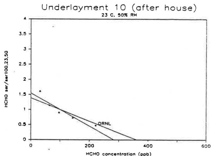
Figure 50. Comparison of Normalized HCHO Emission Rates for Underlayment #10 (third test) to those Predicted by ORNL Emission Model.
