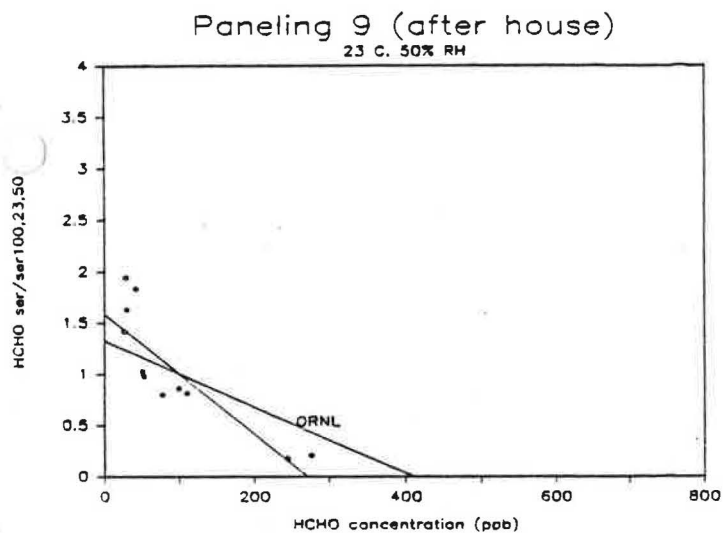
Figure 59. Comparison of Normalized HCHO Emission Rates for Paneling #9 (second test) to those Predicted by ORNL Emission Model.
