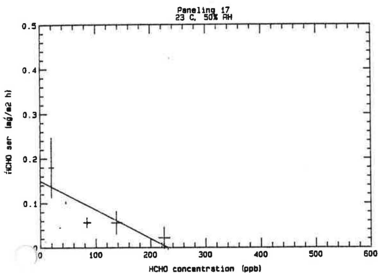
Figure 33. HCHO Emission Rate for Paneling #17 as a Function of HCHO Concentration.*
