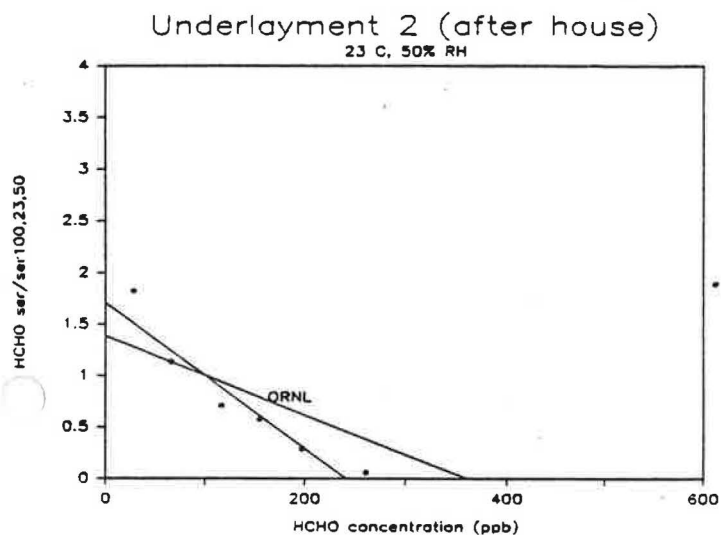
Figure 41. Comparison of Normalized HCHO Emission Rates for Underlayment #2 (third test) to those Predicted by ORNL Emission Model.
