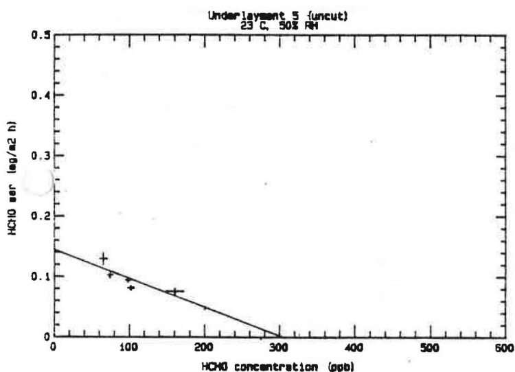
Figure 11. HCHO Emission Rate for Underlayment #5 as a Function of HCHO Concentration (first test).*
