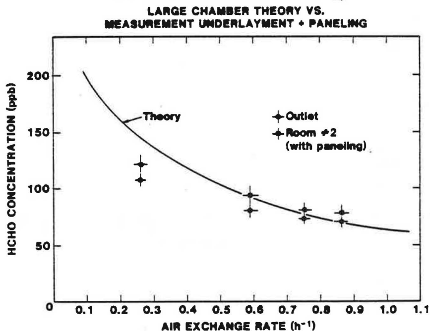
Figure 81. Comparison of Measurements (points) and Predictions of Equation 8 (curve) for Prototype-House Loading of Underlayment and Paneling.*
