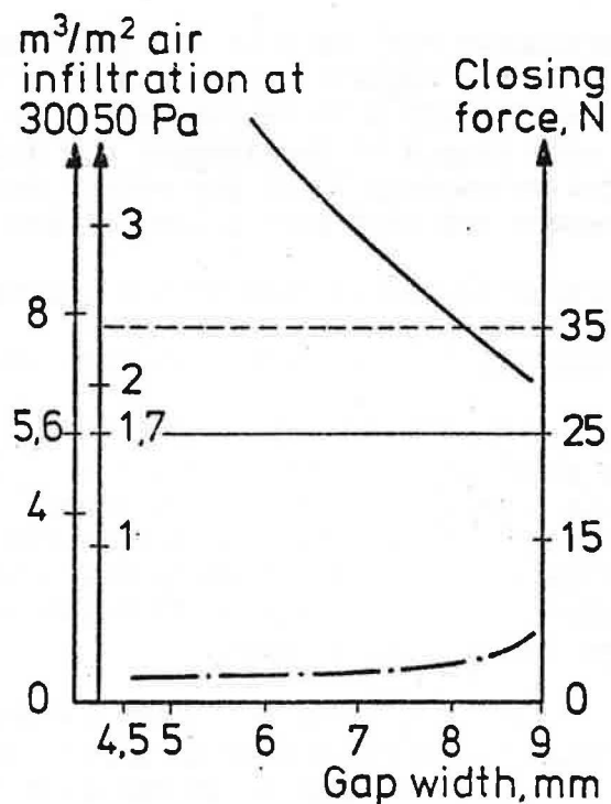
Figure 3. Tubular strips ( h=10 mm, t=0.95 ).
