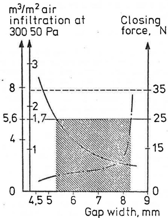
Figure 5. Angle strips ( h=11-12 mm).
