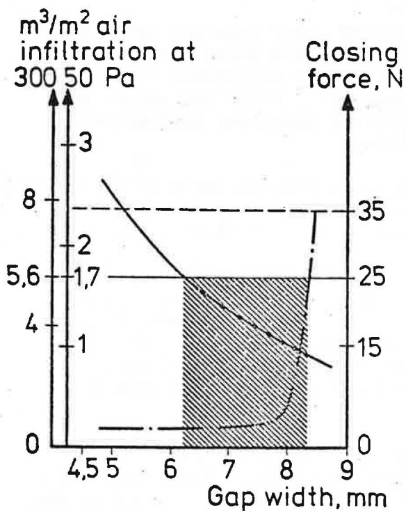
Figure 2. Tubular strips ( h=10 mm, t=0.8 mm).
