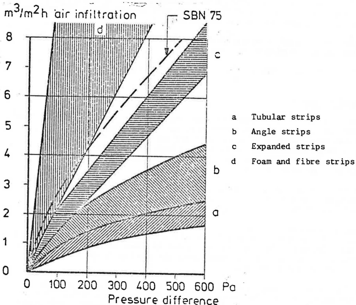
Figure 1. Summary of results for weatherstrips for windows
