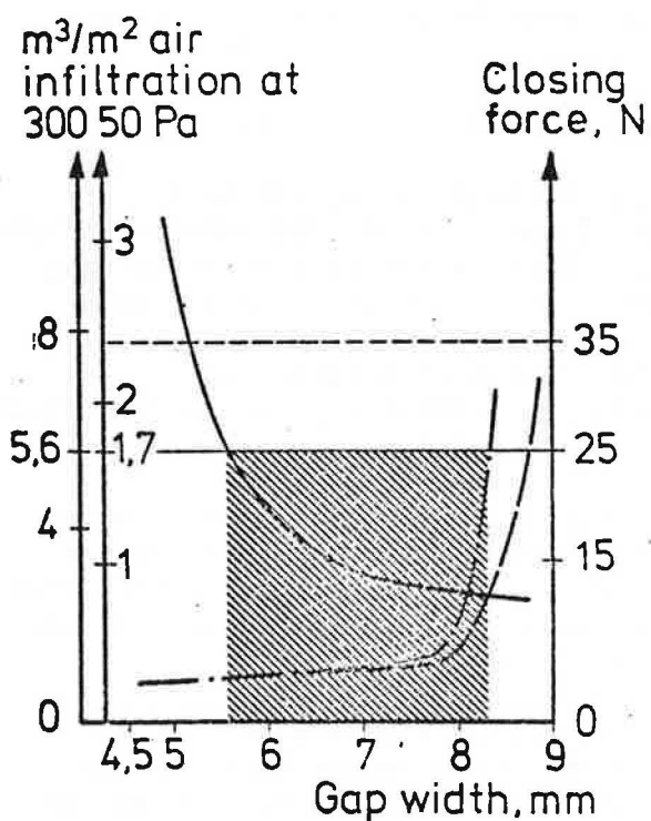
Figure 4. D-strips ( h=10 mm, t=0.6 mm).
